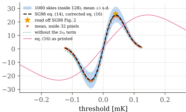
\chi of the full sky
