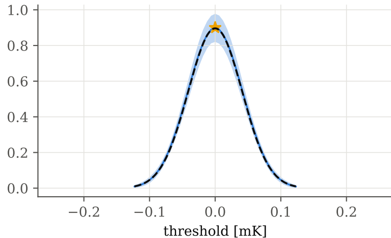
\chi of the full sky
