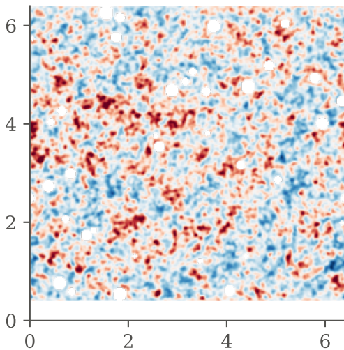
(b) \kappa_E from masked shear
