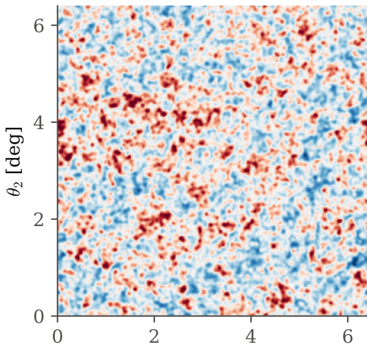
(a) true \kappa
