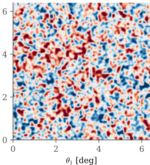
(d) \kappa_E with shape noise, \theta_G = 3'
