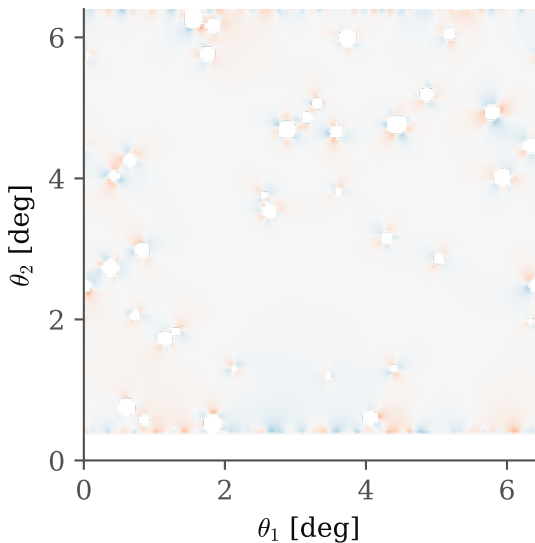
(c) \kappa_B from masked shear
