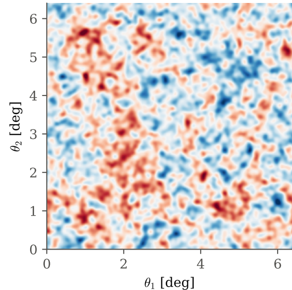
Gaussian: min -0.023, max 0.023
