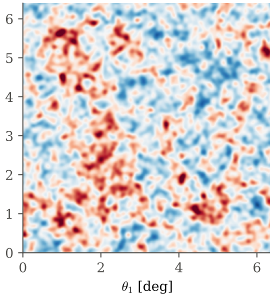
lognormal: min -0.018, max 0.031
