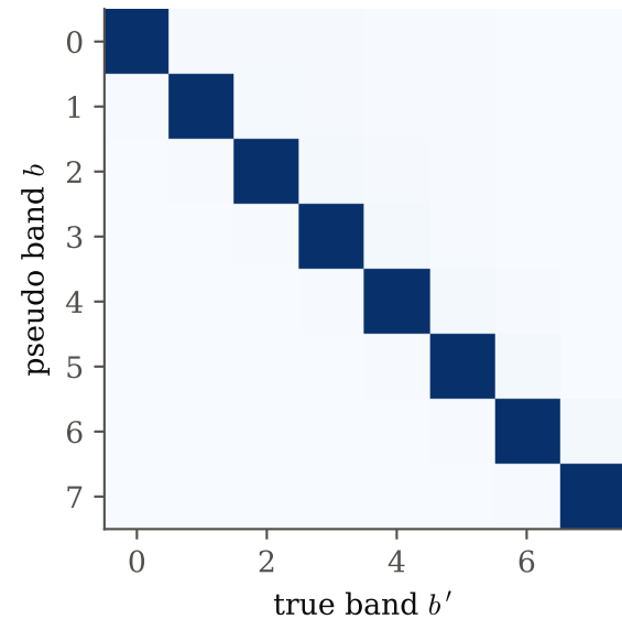
M_{bb'}^{EE} (columns scaled to diagonal 1)
