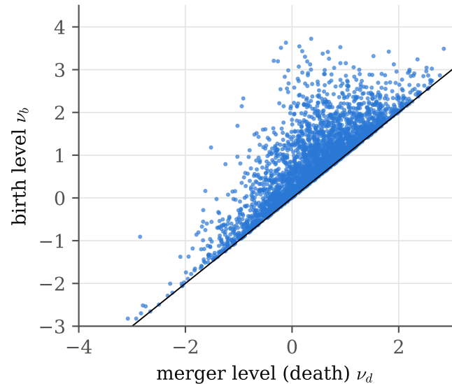
SMICA map, N_{\text{side}} = 128 : 3088 points
