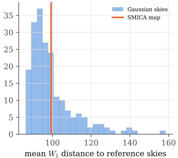
N_{\text{side}} = 128
