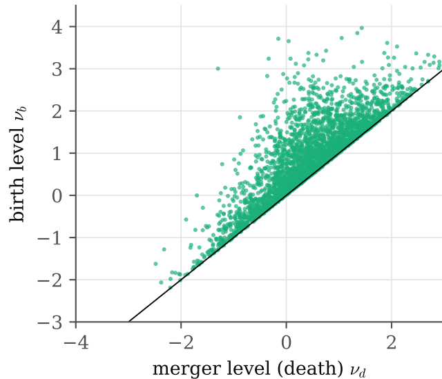
one Gaussian sky, N_{\text{side}} = 128 : 3026 points
