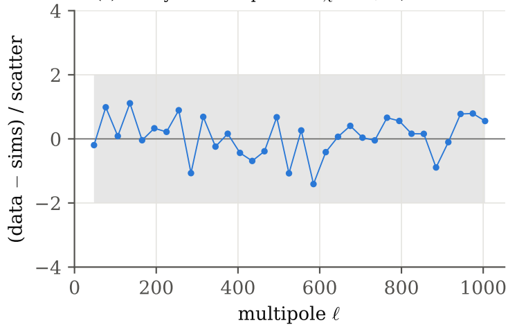
(c) binary mask – apodised: \chi^2 = 15/33 , PTE 1.00
