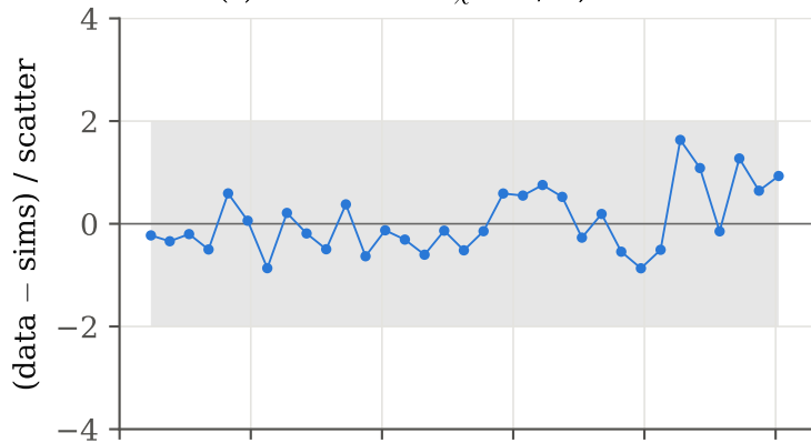
(c) binary mask – apodised: \chi^2 = 15/33 , PTE 1.00
