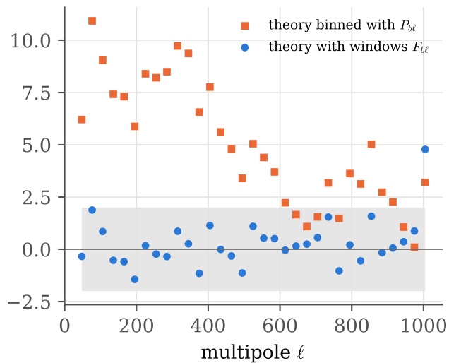
(b) bias test, 400 simulations
