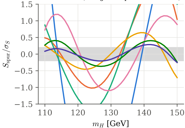
truth: Bern5 (background part of an s+b fit)
