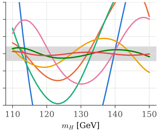
truth: Exp4 (background part of an s+b fit)
