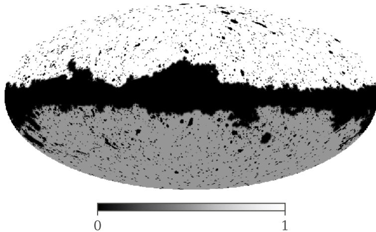
(d) north (white) and south (grey)
