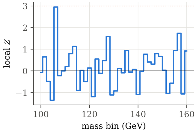
(a) collider: a background-only scan
