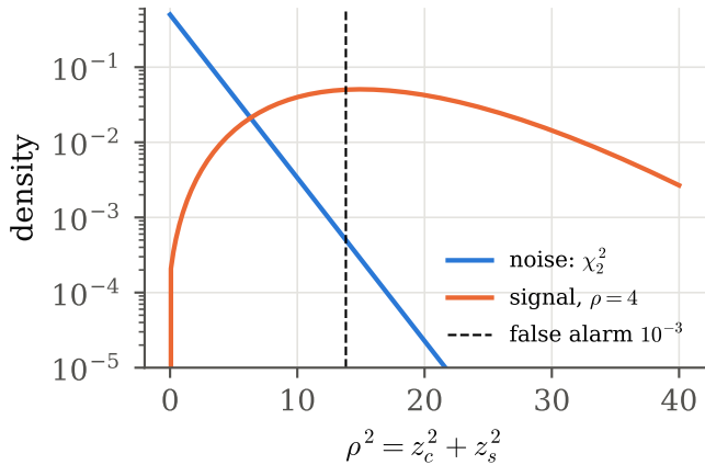
(c) GW: matched filter, unknown phase
