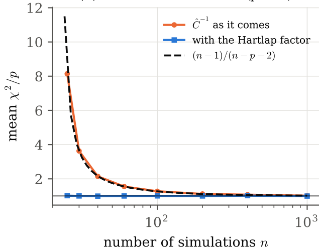
(b) the inverse is biased ( p=20 )
