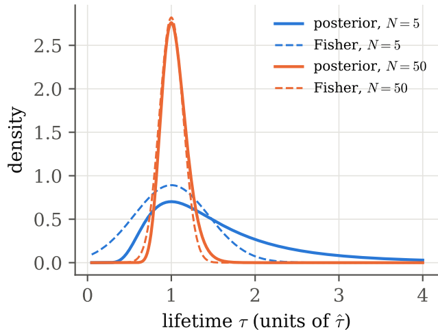
(a) Fisher is not the posterior
