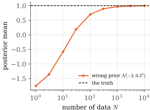
(b) the prior is forgotten only by data
