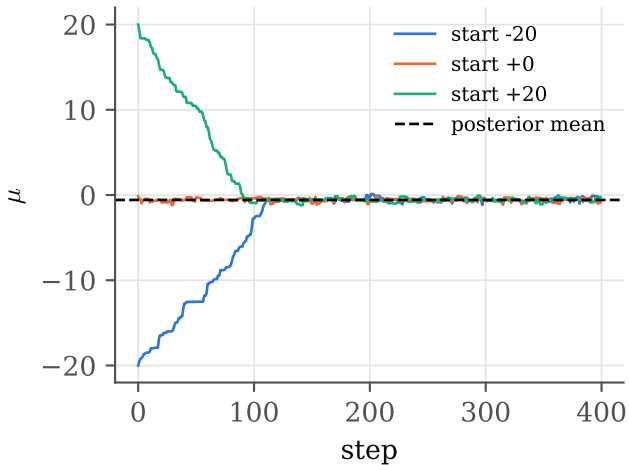
(a) the start is forgotten
