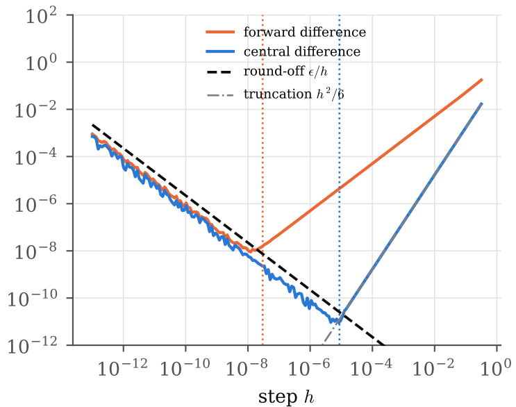
relative error of f'(1) , f = e^x
