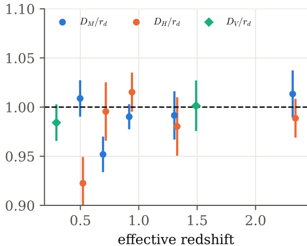
DESI / Planck \Lambda CDM
