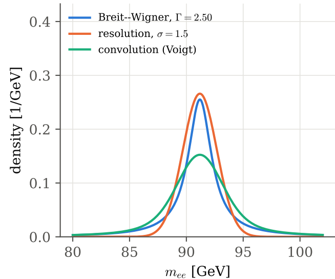
(a) Z: width and resolution comparable
