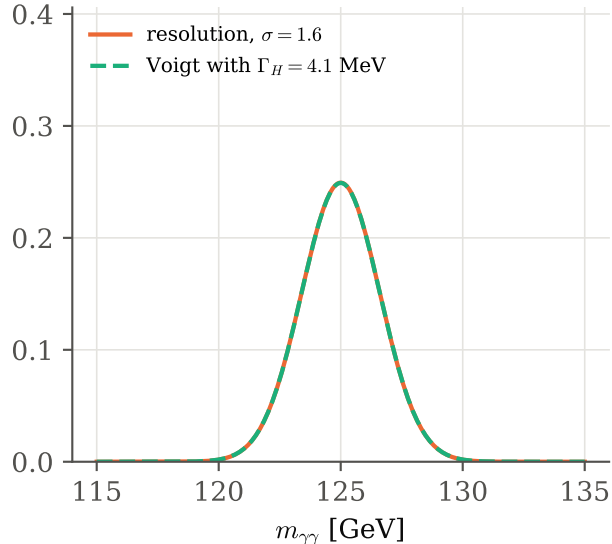
(b) Higgs: resolution only
