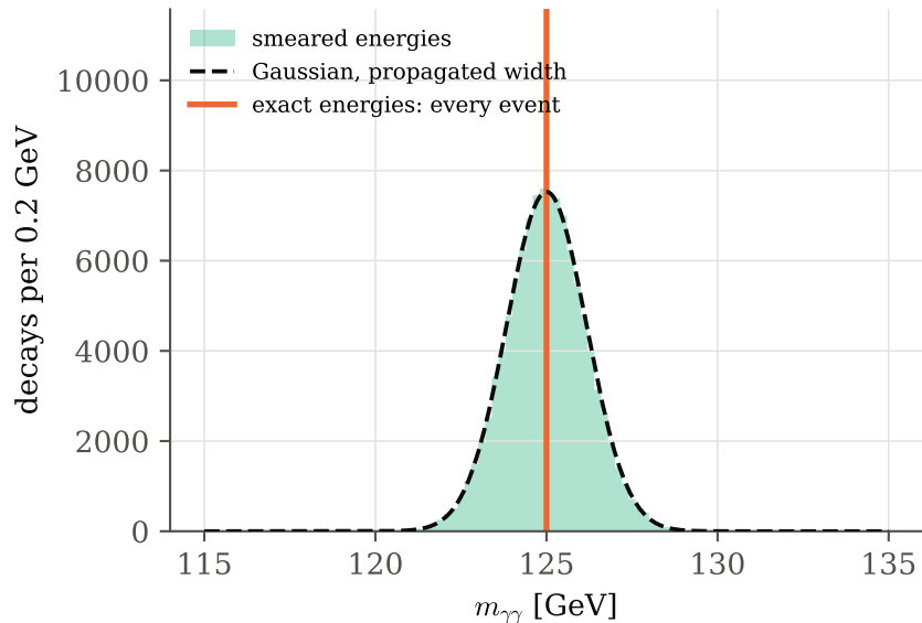
(b) the pair mass is the same in every event
