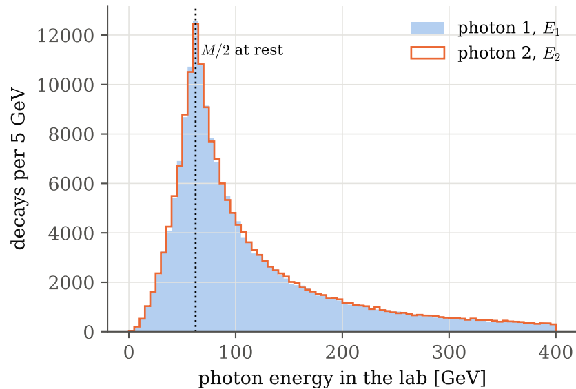
(a) energies depend on the boost
