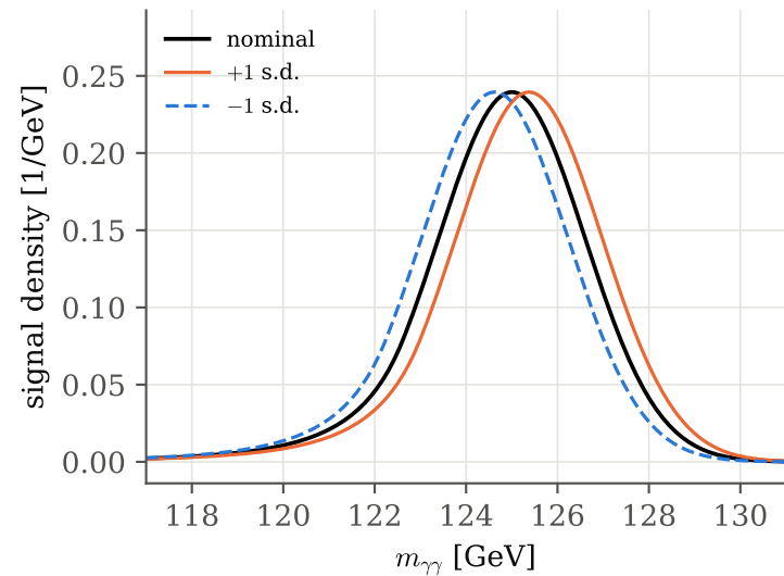
energy scale \pm 0.3\%
