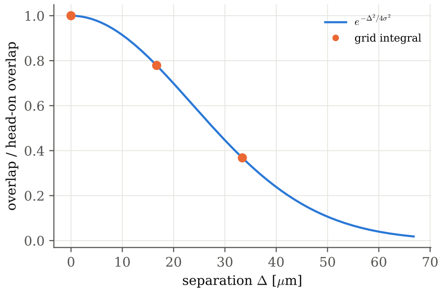
(b) the overlap falls as a Gaussian
