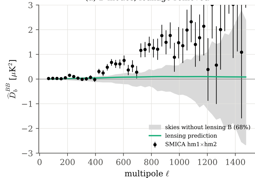
(a) B modes, leakage removed
