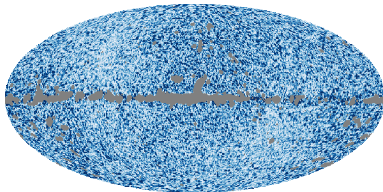
(b) P = \sqrt{Q^2 + U^2} , smoothed 1^\circ
