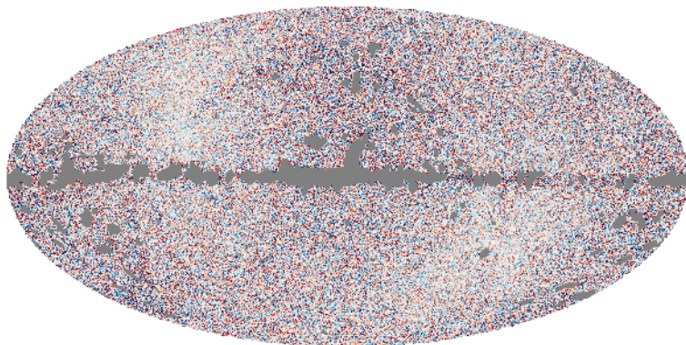
(a) SMICA Q , PMASK
