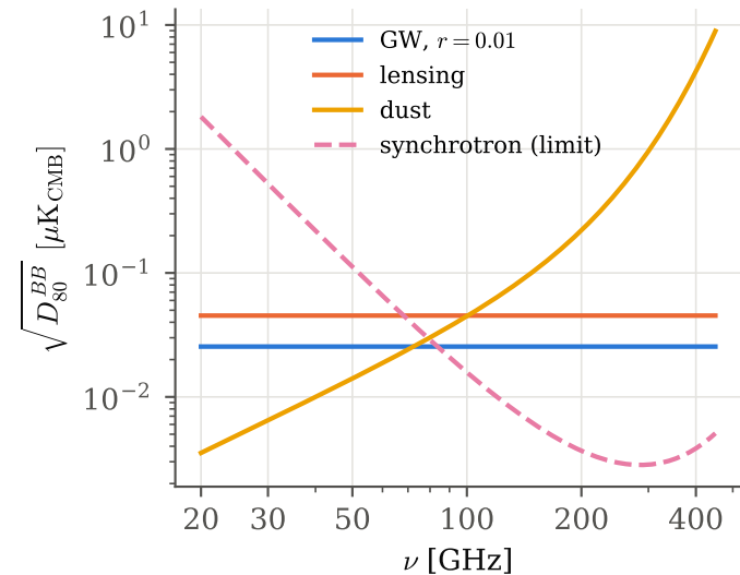
(a) B -mode amplitude at \ell = 80
