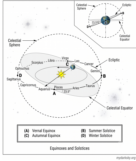
Figure 1.3: The Sun's right ascension and declination change throughout the year as it traces the ecliptic; at the March equinox the Sun lies in the direction of the vernal equinox.
