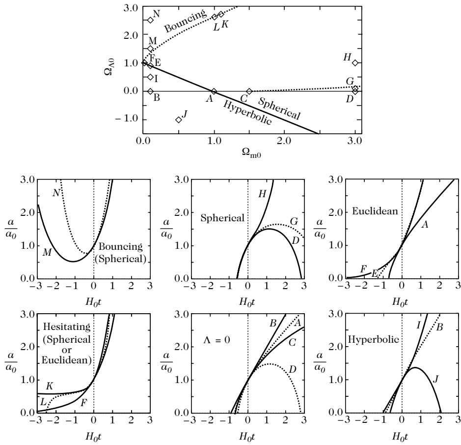
Figure 2.3: Evolution profiles of the cosmic scale factor a(t)/a_0 as a function of H_0 t for various cosmological parameter combinations (\Omega_{m0}, \Omega_{\Lambda0}, K) , illustrating Big Bang, Big Crunch, bouncing, hesitating, and de Sitter asymptotic regimes.
