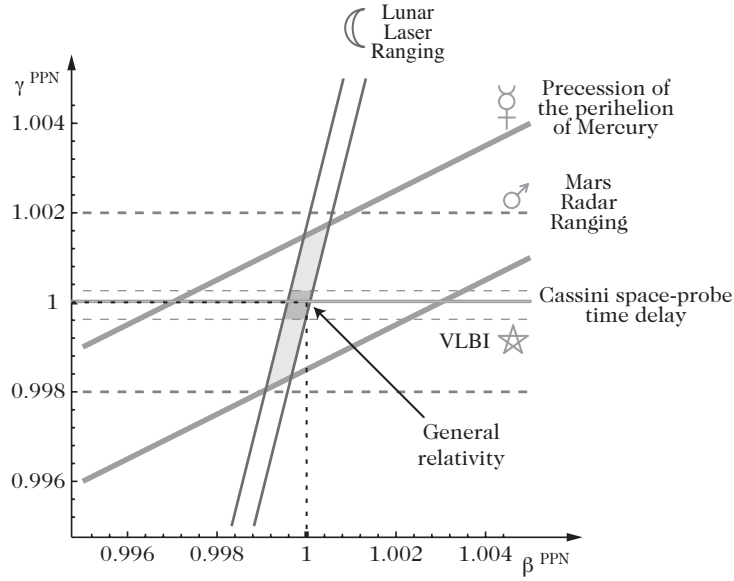
Figure 1.13: Summary of experimental constraints on the Parameterized Post-Newtonian parameters ( \beta_{\text{PPN}}, \gamma_{\text{PPN}} ) in the Solar System. The intersection of bounds from Mercury’s perihelion precession, Lunar Laser Ranging, VLBI light deflection, and the Cassini radio time delay isolates general relativity ( \beta_{\text{PPN}} = \gamma_{\text{PPN}} = 1 ) to high precision.
