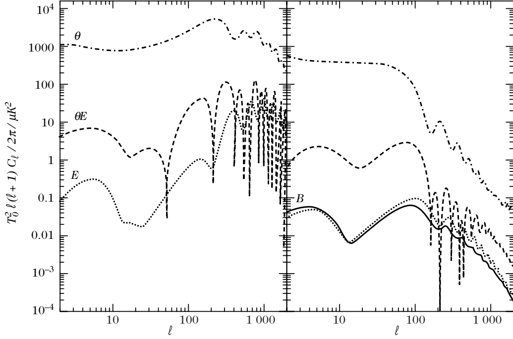
Figure 6.10: The four primary angular power spectra \Theta – \Theta , \Theta – E , E – E , and B – B generated by scalar modes (left panel) and tensor modes (right panel) in an inflationary scenario. Note that the B -mode power spectrum B – B is sourced exclusively by primordial tensor perturbations, while the cross-correlation E – B vanishes identically due to parity conservation.
