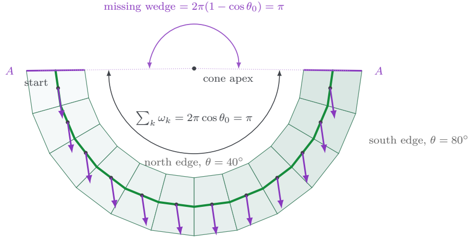
Figure 12.4: Unrolled band of 12 planar facets forming a cone sector: all parallel-transported vectors remain strictly parallel in the Euclidean plane, yielding a net deficit angle \Delta\theta = \pi upon re-gluing the boundary edges A .
