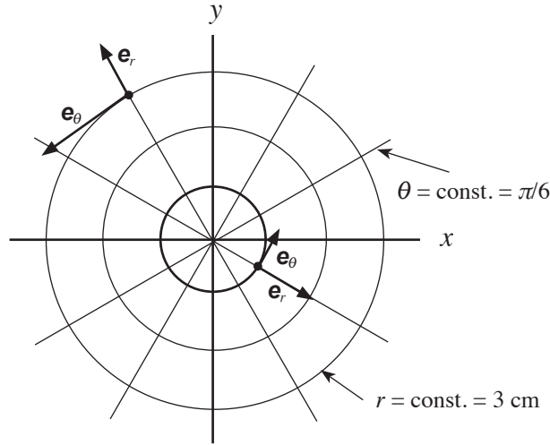
Figure 12.1: The polar-coordinate basis vectors change direction from point to point. Thus, as we move through the coordinate system, the local basis at one point is rotated relative to the basis at another. A vector that is purely radial with respect to one local basis therefore need not remain purely radial when compared with the basis at a neighboring point. The connection coefficients encode precisely this change of the local basis from one point to another, and hence appear in the parallel-transport equation.
