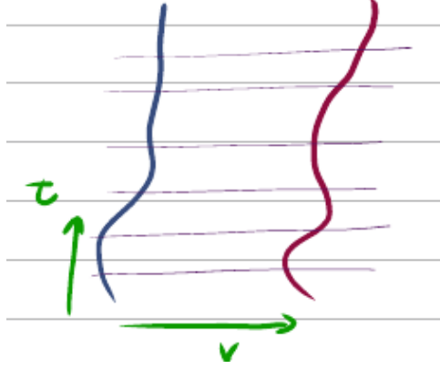
Figure 13.3: A 2-parameter geodesic congruence sheet x^i(\tau, s) with tangent velocity vector u^i = \frac{\partial x^i}{\partial \tau} along the flow and geodesic deviation separation vector v^i = \frac{\partial x^i}{\partial s} across neighboring geodesics.
