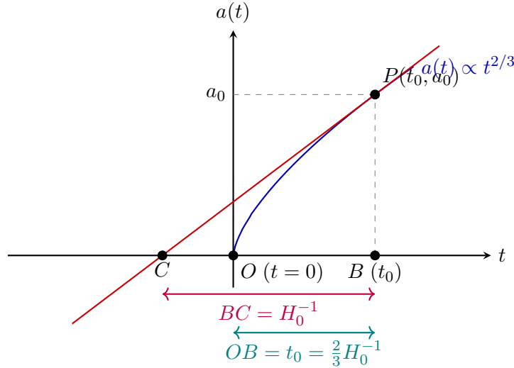
Figure 26.1: Geometric derivation of the cosmic age t_0 for a matter-dominated flat universe. The slope of the tangent line at P(t_0, a_0) is \dot{a}_0 , intercepting the time axis at point C . The distance BC = a_0/\dot{a}_0 = H_0^{-1} represents the Hubble time, yielding t_0 = OB = \frac{2}{3}BC = \frac{2}{3}H_0^{-1} .
