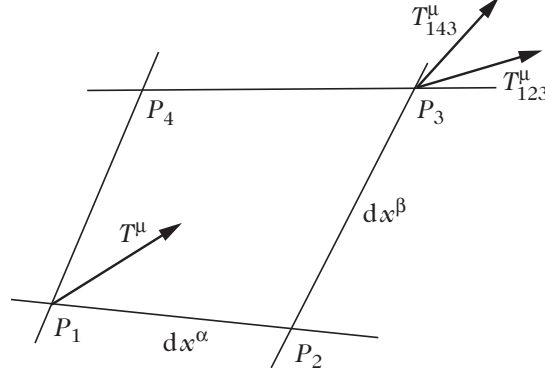
Figure 1.6: The vector T^\mu is parallel transported along the path P_1 \rightarrow P_3 passing either through P_2 (yielding T^\mu_{123} ) or through P_4 (yielding T^\mu_{143} ). These two vectors coincide if and only if the Riemann curvature tensor vanishes.
