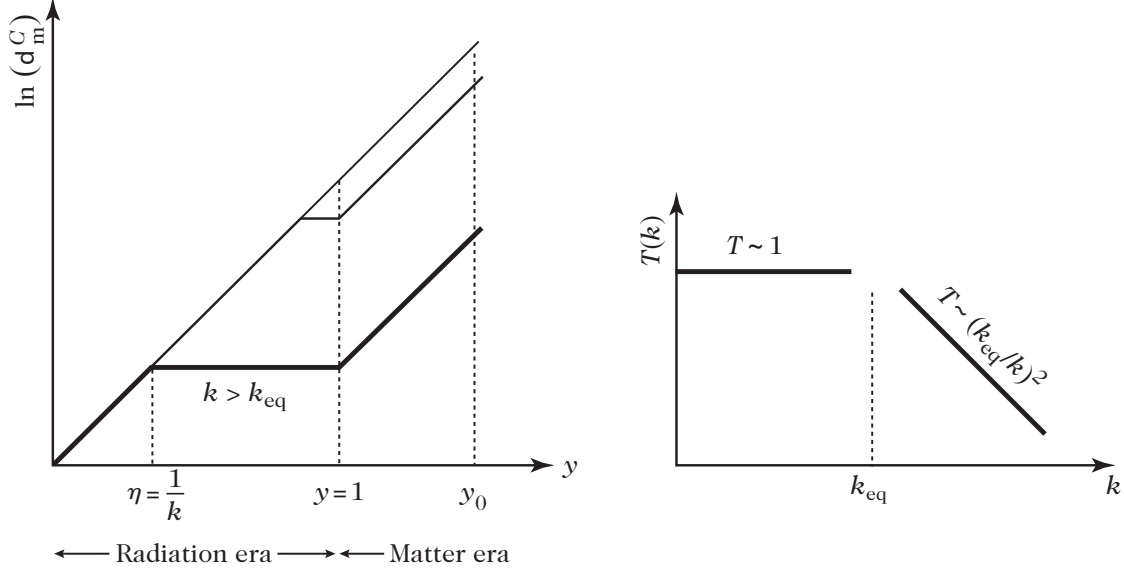
Figure 4.15: (left): Modes that become sub-Hubble during the radiation-dominated era ( k > k_{eq} ) remain nearly constant (neglecting logarithmic growth) from \eta \sim 1/k to \eta \sim 1/k_{eq} . (right): The amplitude of the density contrast on these scales suffers from a suppression factor of order (k_{eq}/k)^2 . For k > k_{eq} one therefore expects the transfer function to scale as T \propto (k_{eq}/k)^2 , while remaining of order unity for k < k_{eq} .
