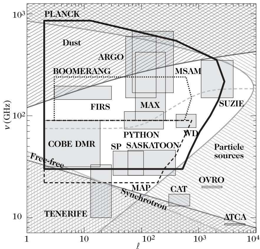
Figure 6.13: Angular and frequency sensitivity ranges for major ground-based, sub-orbital, and space CMB experiments. The shaded regions denote frequency regimes where Galactic foreground emissions (synchrotron, free-free, and thermal dust) exceed 20 \mu\text{K} in the cleanest 20% of the sky. From Ref. [53].
