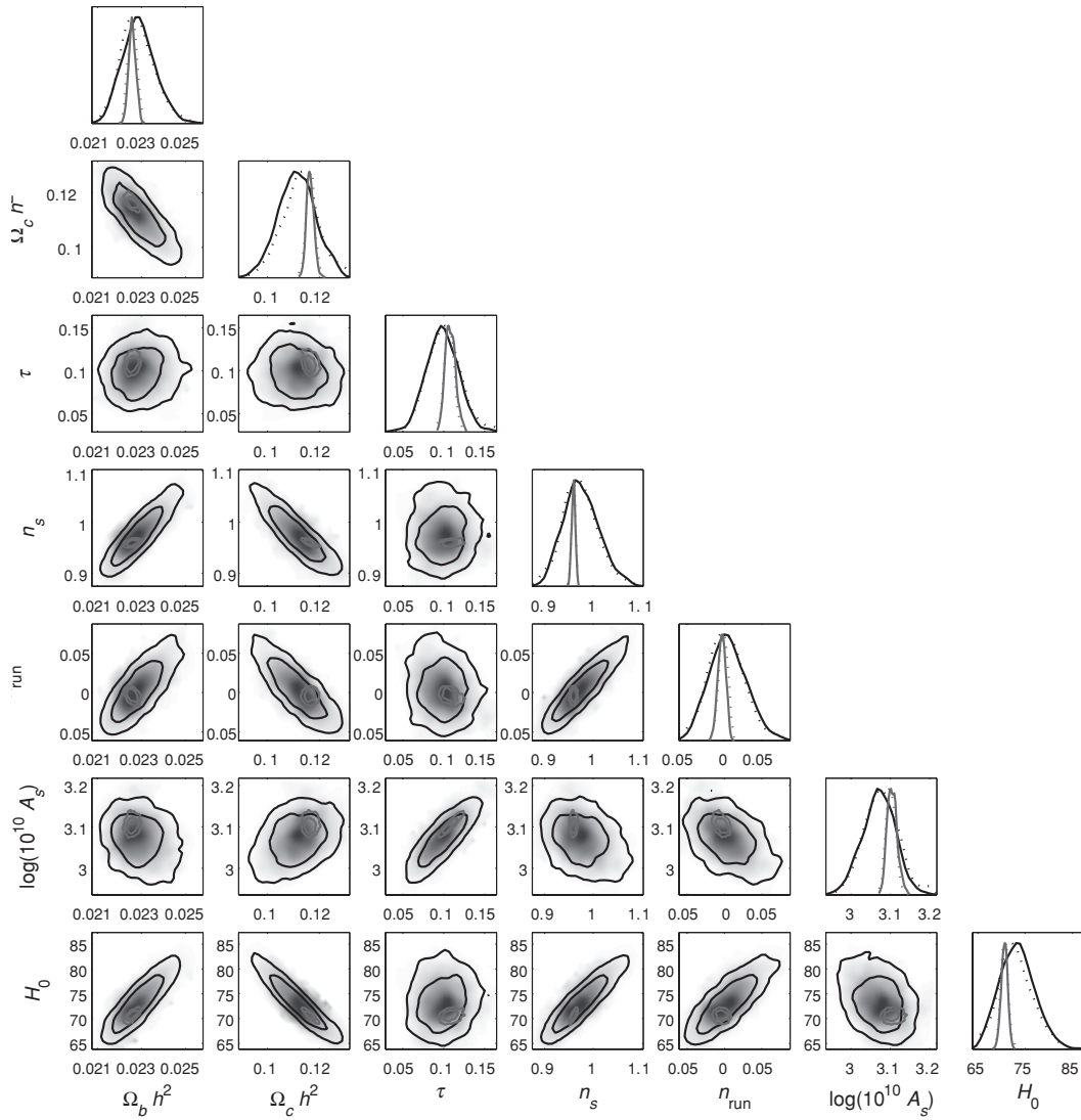
Figure 7.10: Marginalized 1D and 2D parameter probability distributions forecasted for the Planck satellite experiment for a 7-parameter flat model ( \Omega_b h^2, \Omega_{\text{cdm}} h^2, \tau, n_s, n_{\text{run}}, \ln(10^{10} A_s), H_0 ). Figure from ESA (2005).
