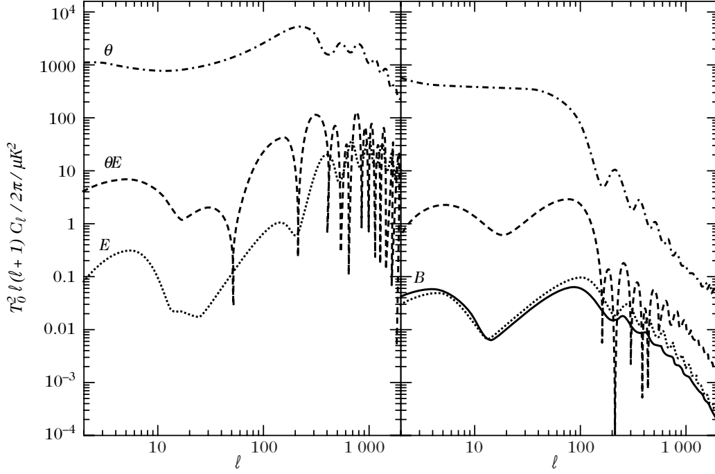
Figure 6.10: The four primary angular power spectra \Theta\text{--}\Theta , \Theta\text{--}E , E\text{--}E , and B\text{--}B generated by scalar modes (left panel) and tensor modes (right panel) in an inflationary scenario. Note that the B -mode power spectrum B\text{--}B is sourced exclusively by primordial tensor perturbations, while the cross-correlation E\text{--}B vanishes identically due to parity conservation.
