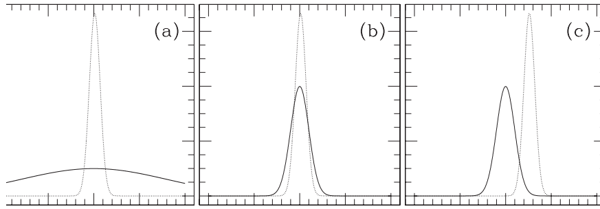
Figure 7.11: Three 1-parameter models with their prior (solid lines) and posterior (dotted curves). All three models have comparable maximum likelihoods. In (a), the prior volume is much wider than the posterior, leading to a small Occam factor. In (b) and (c), the widths are comparable, but model (c) lacks overlap between prior and data. Model (b) has the largest Bayesian evidence.
