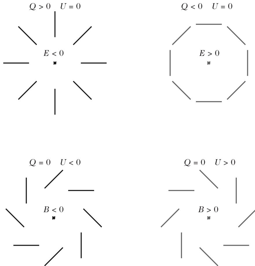
Figure 6.6: Polarization field configurations representing pure E -mode and pure B -mode patterns in the vicinity of a given central point. The line segments indicate the local orientation and amplitude of the linear polarization, directly depicting the Stokes parameters Q and U . These patterns repeat periodically across the plane. Because the scalar E and pseudo-scalar B fields are related to Q and U non-locally, determining their amplitudes at a specific point requires sampling the surrounding polarization texture. Under spatial reflection across a coordinate axis, the two upper configurations ( E -modes) are invariant, whereas the two lower configurations ( B -modes) are interchanged under reflection, illustrating their opposite parity properties.
