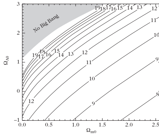
Figure 2.8: Isocontours of the present cosmic age t_0 (in units of 10^9 yr) in the (\Omega_{m0}, \Omega_{\Lambda0}) plane. The shaded region denotes non-singular bouncing models lacking a past Big Bang.
