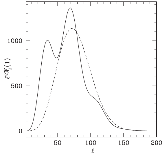
Figure 7.4: The window function \ell^2 W_\ell(1) for a differencing beam of width \sigma = 1^\circ for two different throw values: x_0 = 4^\circ (solid line) and x_0 = 1^\circ (dashed line). The high- \ell cutoff at \ell \sim 70 is dictated by the Gaussian beam width \sigma . When the throw x_0 differs from \sigma , a second low- \ell modulation appears on the left corresponding to the angular throw scale.
