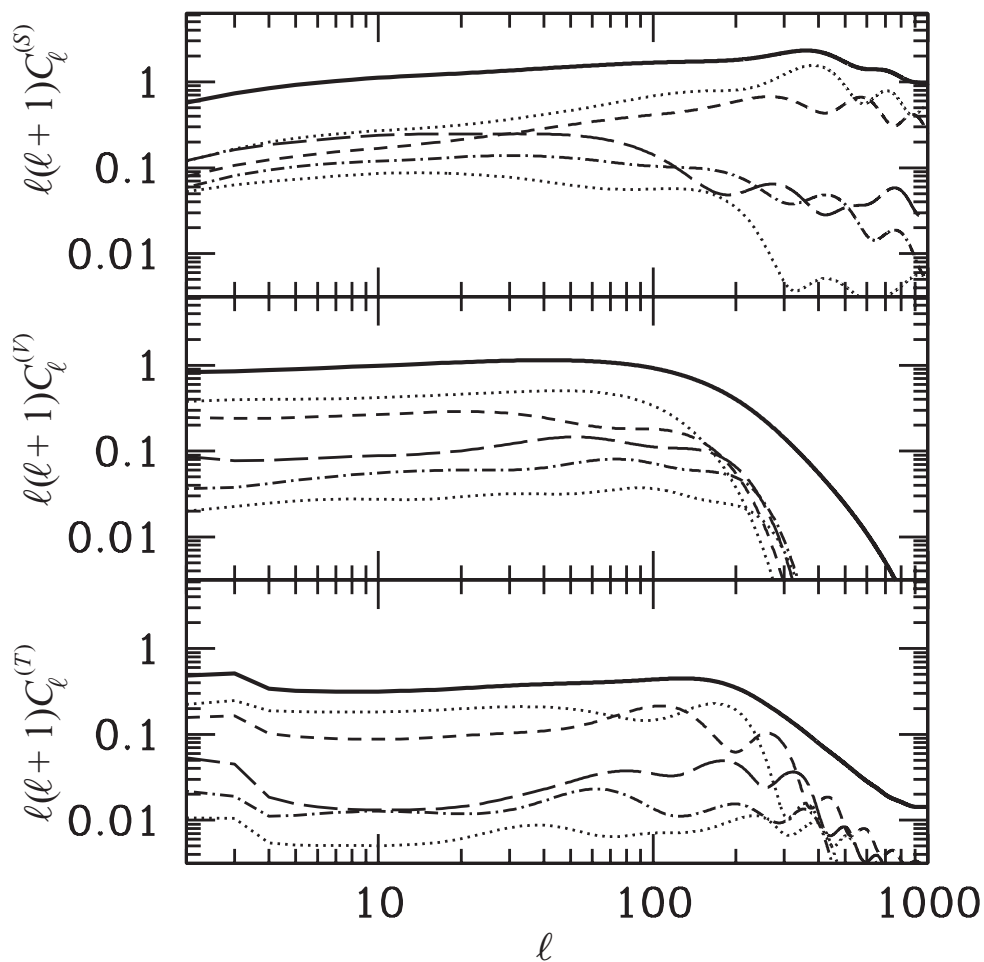
Figure 7.21: The scalar ( S ), vector ( V ), and tensor ( T ) contributions to the CMB temperature power spectrum \ell(\ell+1)C_\ell for a 4-component global texture model. Dashed curves indicate contributions from individual single eigenfunctions, while the bold solid curve shows their total sum over 100 modes. While individual eigenmodes display oscillations, they wash out into a broad hump in the sum (data courtesy of Bevis et al., 2004).
