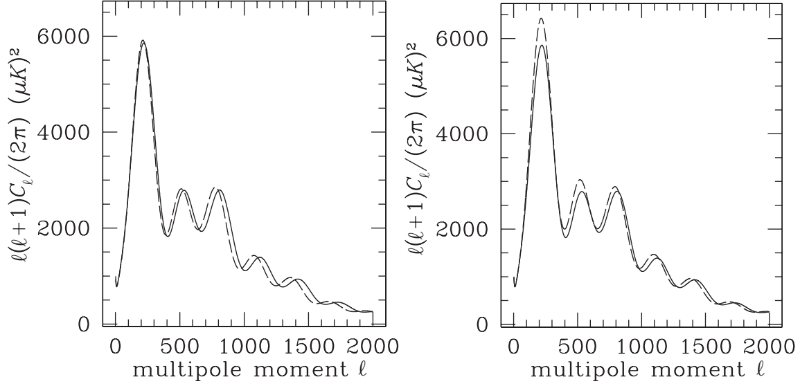
Figure 7.3: The CMB power spectrum for massless neutrinos and massive neutrinos with mass m_\nu = 2 \text{ eV} (dashed lines). Left: Cold dark matter density \Omega_{\text{cdm}}h^2 = 0.12 is fixed. Right: Total matter density \Omega_{\text{m}}h^2 = 0.144 is fixed. In all curves, \Omega_{\text{tot}} = 1 , \Omega_{\text{b}}h^2 = 0.022 , and h = 0.7 . At fixed \Omega_{\text{m}}h^2 , massive neutrinos mimic a lower matter density because they are not yet fully non-relativistic at decoupling.
