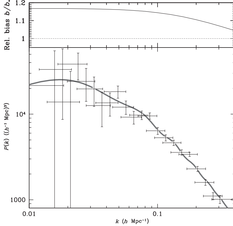
Figure 7.14: The galaxy power spectrum from the Sloan Digital Sky Survey (SDSS) corrected by the modeled galaxy bias (top). The solid curve represents the best-fitting linear \Lambda CDM cosmological model (adapted from Tegmark et al., 2004).
