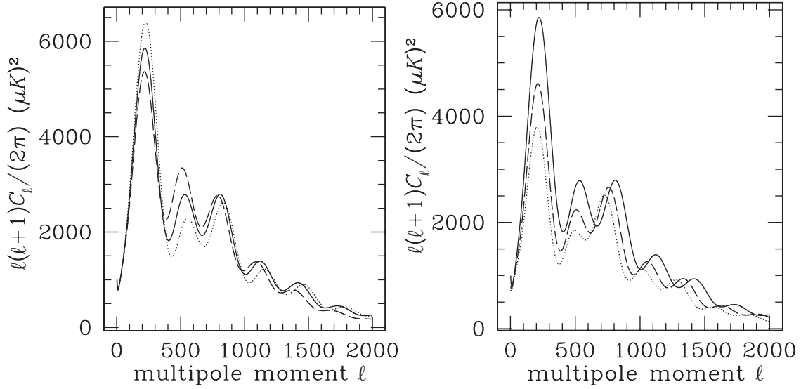
Figure 7.2: Left: The asymmetry of even and odd acoustic peaks and its dependence on \Omega_b h^2 . The temperature power spectrum is plotted for \Omega_b h^2 = 0.02 (solid line), \Omega_b h^2 = 0.03 (dotted line), and \Omega_b h^2 = 0.01 (dashed line). Right: Fixing \Omega_b h^2 = 0.02 and varying the physical matter density: \Omega_m h^2 = 0.12 (solid), \Omega_m h^2 = 0.20 (dashed), and \Omega_m h^2 = 0.30 (dotted). Higher \Omega_m h^2 increases peak asymmetry, while smaller \Omega_m h^2 boosts the first peak via the early integrated Sachs–Wolfe effect.
