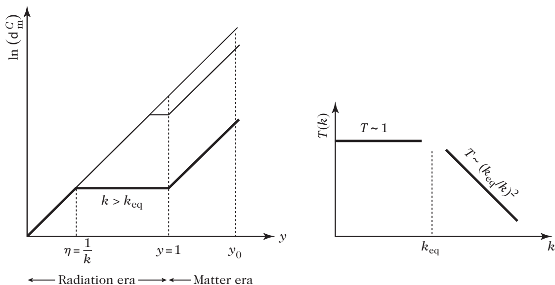
Figure 4.15: (left): Modes that become sub-Hubble during the radiation-dominated era ( k > k_{\text{eq}} ) remain nearly constant (neglecting logarithmic growth) from \eta \sim 1/k to \eta \sim 1/k_{\text{eq}} . (right): The amplitude of the density contrast on these scales suffers from a suppression factor of order (k_{\text{eq}}/k)^2 . For k > k_{\text{eq}} one therefore expects the transfer function to scale as T \propto (k_{\text{eq}}/k)^2 , while remaining of order unity for k < k_{\text{eq}} .
