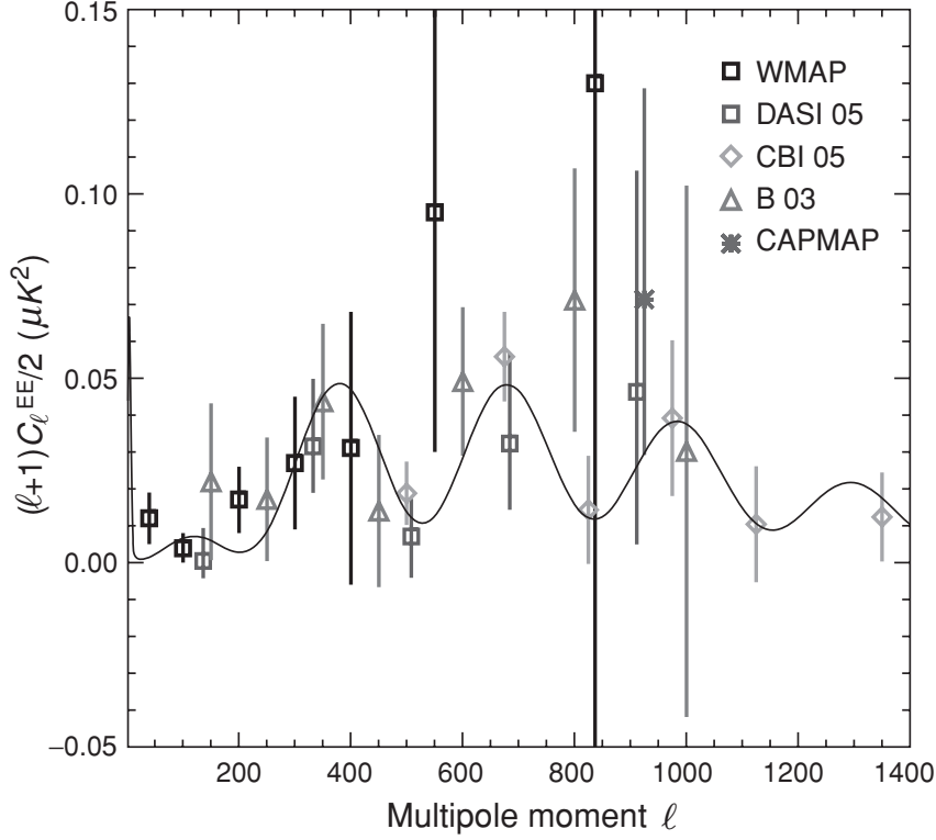
Figure 7.7: The measured EE polarization power spectrum from the WMAP 3-year data, BOOMERanG, DASI, CBI, and CAPMAP experiments (from Page et al., 2007).
