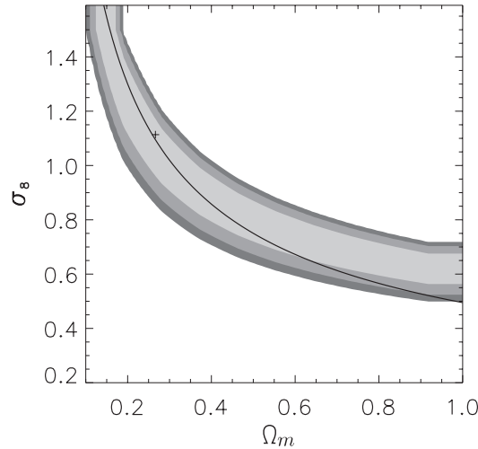
Figure 7.17: Cosmological constraints in the (\Omega_m, \sigma_8) plane from cosmic shear measurements (Maoli et al., 2001). The light, medium, and dark shaded regions enclose the 1\sigma , 2\sigma , and 3\sigma confidence contours. The cross marks the best-fit model, and the solid curve displays the constraint inferred from local galaxy cluster abundances.
