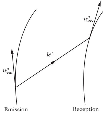
Figure 1.8: A photon emitted with wavevector k^\mu by an observer with 4-velocity u_{em}^\mu travels along a null geodesic to an observer with 4-velocity u_{rec}^\mu .
