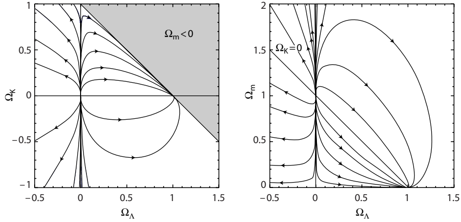
Figure 2.4: Phase space trajectories of the cosmological dynamical system in the (\Omega_K, \Omega_\Lambda) plane (left) and (\Omega_m, \Omega_\Lambda) plane (right) for dust ( \gamma = 1, w = 0 ). Arrows indicate the direction of cosmic time evolution.
