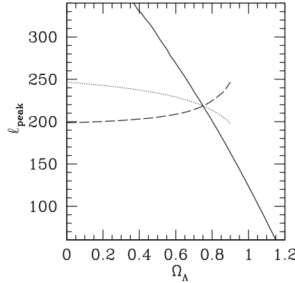
Figure 7.1: The position of the first acoustic peak \ell_1 as a function of \Omega_\Lambda . Solid line: varying \Omega_K while leaving all other parameters fixed. Dashed line: varying \Omega_\Lambda at fixed h = 0.72 . Dotted line: varying \Omega_\Lambda at fixed \Omega_m h^2 . The fixed baseline parameters are \Omega_K = 0, h = 0.72, \Omega_b h^2 = 0.022, \Omega_m = 0.25, n_s = 0.96, \tau_{\text{ri}} = 0.085 , so that all curves intersect at \Omega_\Lambda = 0.75 . Notice the pronounced sensitivity of \ell_1 to spatial curvature.
