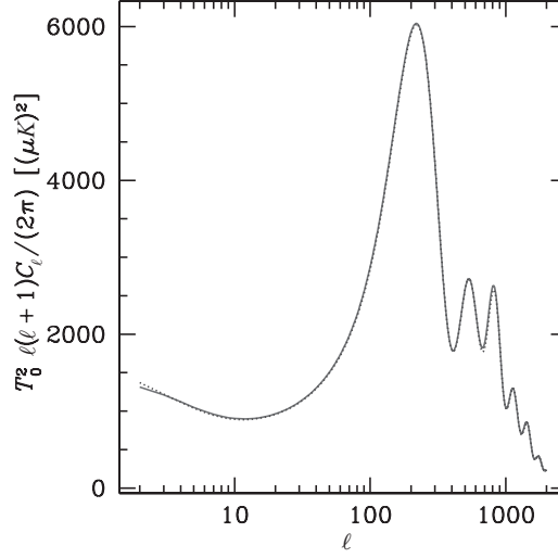
Figure 7.13: Comparison between a purely scalar model with red tilt n_s = 0.96 (solid line) and a model with a significant tensor contribution of r = 0.3 and scale-invariant tilt n_s = 1.0 (dotted line). Both models lie within 1\sigma – 2\sigma of concordance parameters and produce nearly identical temperature power spectra.
