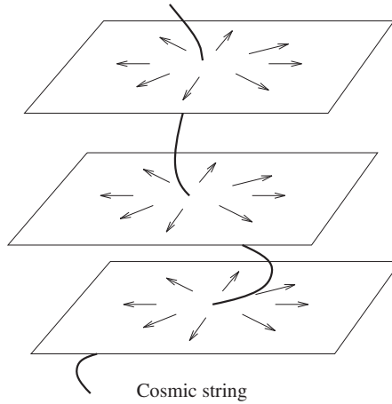
Figure 7.19: A cosmic string in 3D space with the corresponding spatial configuration of the complex Higgs field indicated by arrows.
