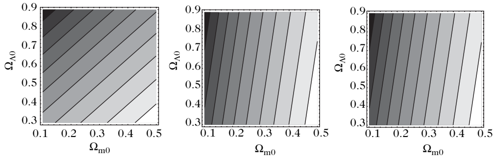
Figure 2.7: Isocontours of the normalized expansion rate function E(z) in the (\Omega_{m0}, \Omega_{\Lambda0}) plane at redshifts z = 1 (left), z = 3 (middle), and z = 10 (right). The degeneracy directions rotate with redshift, demonstrating how multi-epoch observations break cosmological parameter degeneracies.
