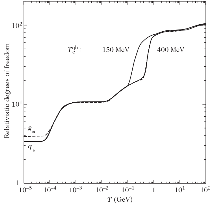
Figure 3.7: Evolution of the effective relativistic degrees of freedom g_*(T) and g_{*S}(T) as a function of temperature T in the Standard Model SU(3)_c \times SU(2)_L \times U(1)_Y , showing the electroweak, quark-hadron QCD ( T_c \approx 150\text{--}400 MeV), and e^+e^- annihilation steps.
