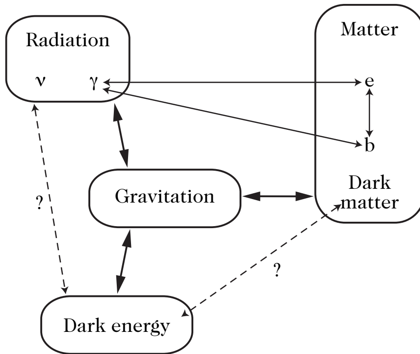
Figure 4.10: The cosmological fluid components and their interactions. Baryons and electrons are tightly coupled through the Coulomb interaction, while photons couple to charged matter via Compton scattering. Dark matter is assumed to interact with ordinary baryonic matter solely through gravity. It is not excluded that dark energy may interact with ordinary matter or with dark matter through an as yet unknown physical mechanism.
