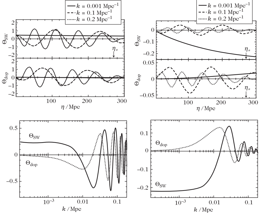
Figure 5.4: Evolution of \Theta_{\text{SW}} = \delta_\gamma^N/4 + \Phi and of \Theta_{\text{dop}} \sim kV_\gamma/\sqrt{3} as a function of time for three modes with wavenumber k = 10^{-3} (solid line), 10^{-1} (dashed) and 2 \times 10^{-1} \text{ Mpc}^{-1} (dotted). The contribution at the time of decoupling as a function of k is presented at the bottom. We compare the adiabatic (left) to the isocurvature (right) initial conditions.
