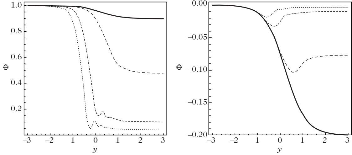
Figure 4.12: Evolution of the gravitational potential for k = 10^{-2}, 0.1, 0.5, 1 \text{ Mpc}^{-1} for adiabatic (left) and isocurvature (right) initial conditions. These curves should be compared with Fig. 4.9, for which entropy fluctuations were neglected.
