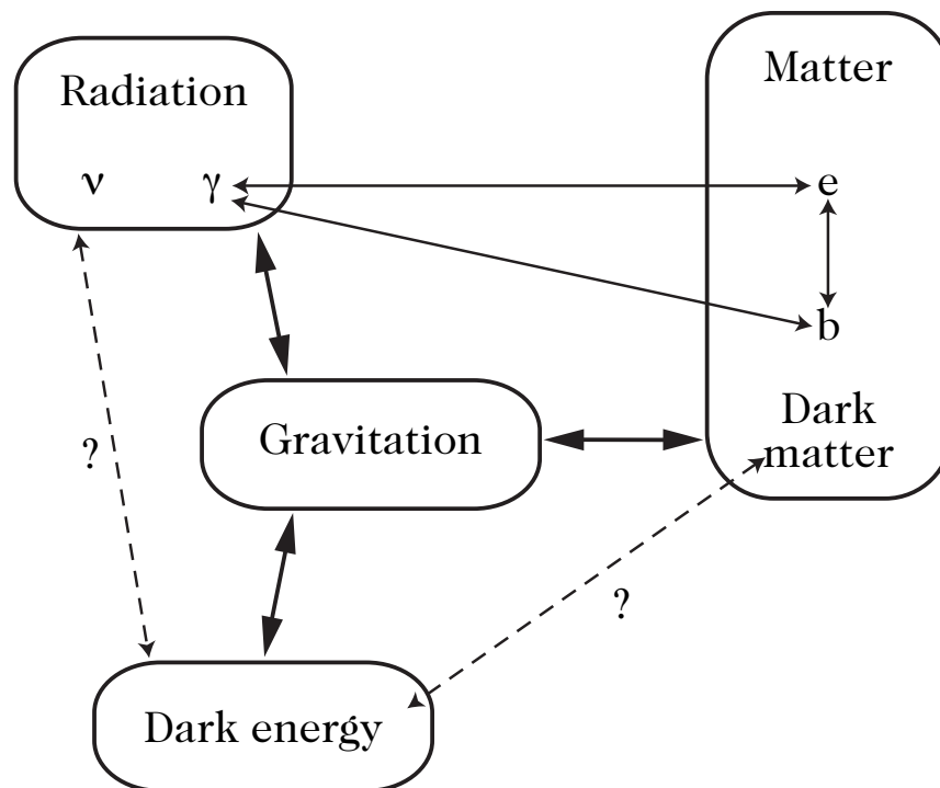
Figure 4.10: The cosmological fluid components and their interactions. Baryons and electrons are tightly coupled through the Coulomb interaction, while photons couple to charged matter via Compton scattering. Dark matter is assumed to interact with ordinary baryonic matter solely through gravity. It is not excluded that dark energy may interact with ordinary matter or with dark matter through an as yet unknown physical mechanism.
