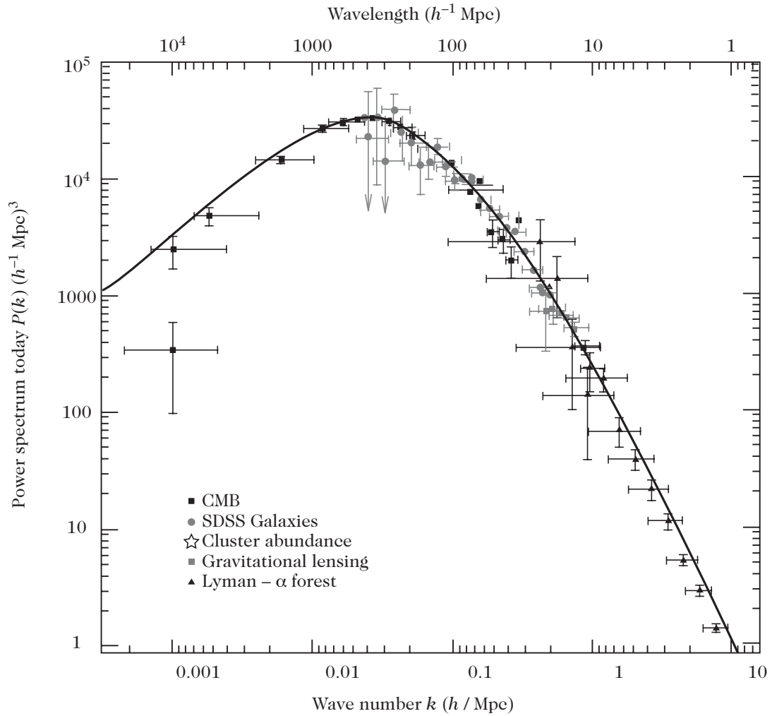
Figure 4.20: The matter power spectrum compared with various observational constraints, ranging from linear scales (cosmic microwave background) to non-linear scales (galaxy surveys, here SDSS), cluster abundances, gravitational lensing, and Lyman- \alpha forests. From (4.4.42) we get the transfer function which can be used P_m = P_\delta T^2(k) D^2(z) , where P_\delta \propto k .
