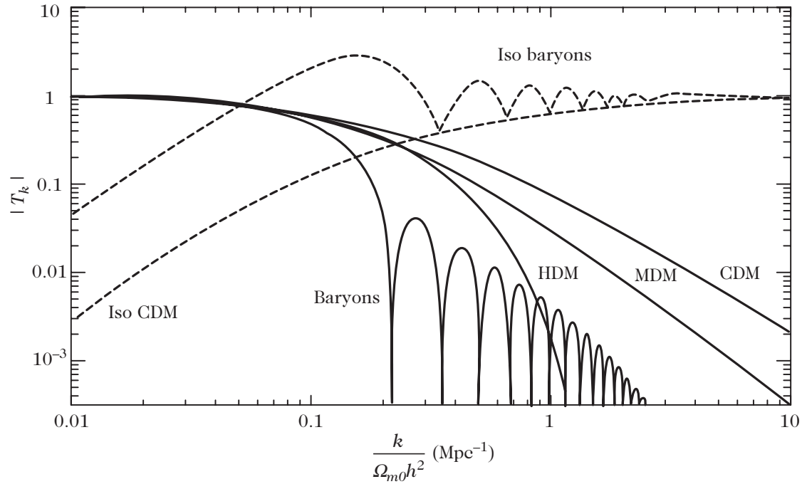
Figure 4.18: Transfer function for different cosmological dark-matter scenarios. The overall shape of this transfer function can be understood directly from the analytical considerations presented above, cf. (4.4.41). From Ref. [8].
