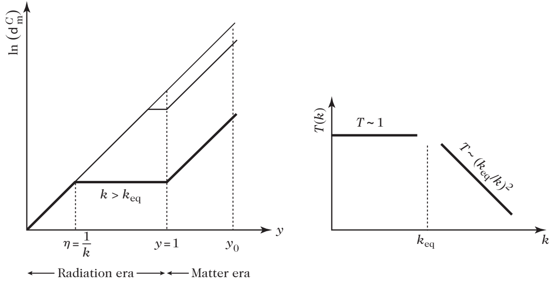
Figure 4.17: (left): Modes that become sub-Hubble during the radiation-dominated era ( k > k_{eq} ) remain nearly constant (neglecting logarithmic growth) from \eta \sim 1/k to \eta \sim 1/k_{eq} . (right): The amplitude of the density contrast on these scales suffers from a suppression factor of order (k_{eq}/k)^2 . For k > k_{eq} one therefore expects the transfer function to scale as T \propto (k_{eq}/k)^2 , while remaining of order unity for k < k_{eq} .
