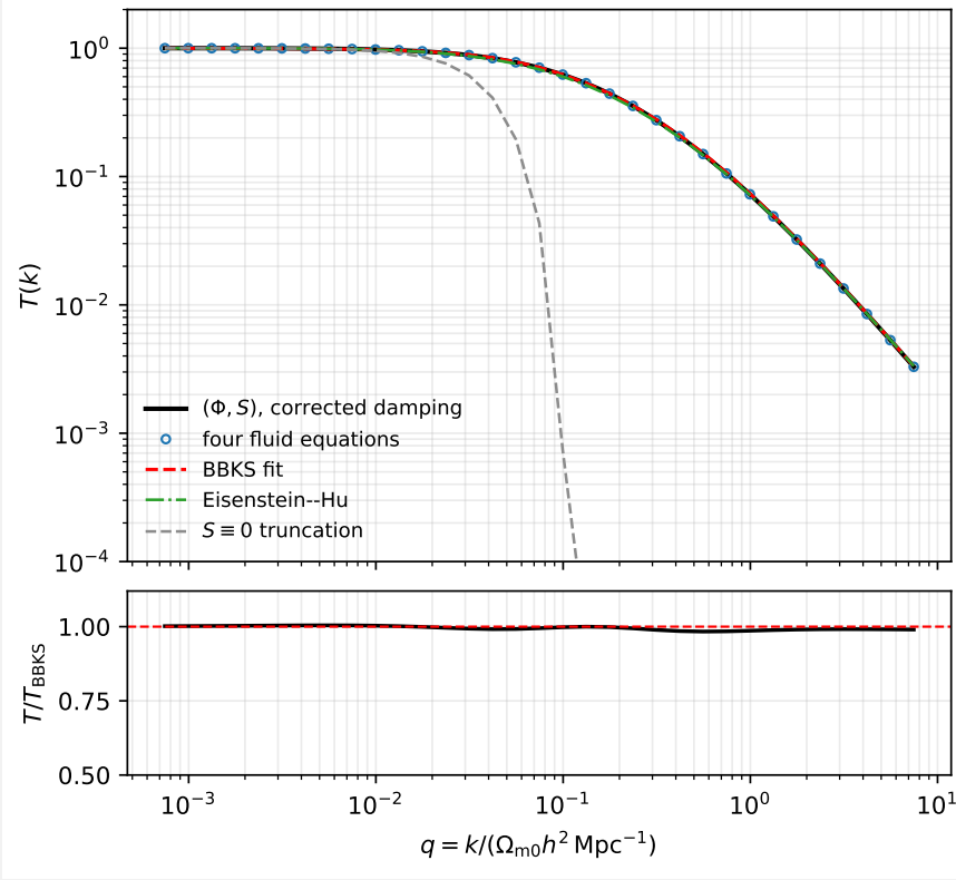
Figure 4.16: Transfer function from the system (14) (solid) and from the fluid equations (6) (circles), against the fitting formula (4.4.42), the Eisenstein–Hu zero-baryon form, the same system integrated with the damping coefficient (3y + 2)/[2y(1 + y)] (dotted), and the truncation S \equiv 0 (grey dashed). Lower panel: ratio to (4.4.42).
