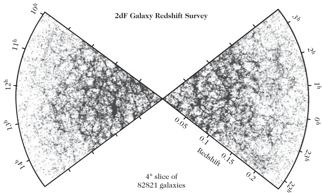
Figure 4.19: The distribution of galaxies across a 4^\circ -wide slice from the 2dFGRS survey catalogue. Such observations of the large-scale structure of the Universe provide the empirical foundation for measurements of the matter power spectrum.
