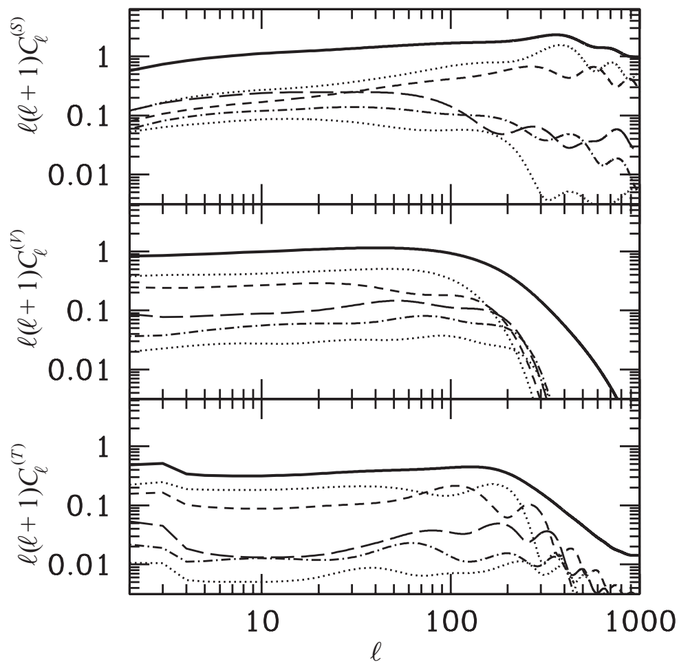
Figure 7.21: The scalar ( S ), vector ( V ), and tensor ( T ) contributions to the CMB temperature power spectrum \ell(\ell+1)C_\ell for a 4-component global texture model. Dashed curves indicate contributions from individual single eigenfunctions, while the bold solid curve shows their total sum over 100 modes. While individual eigenmodes display oscillations, they wash out into a broad hump in the sum (data courtesy of Bevis et al., 2004).
