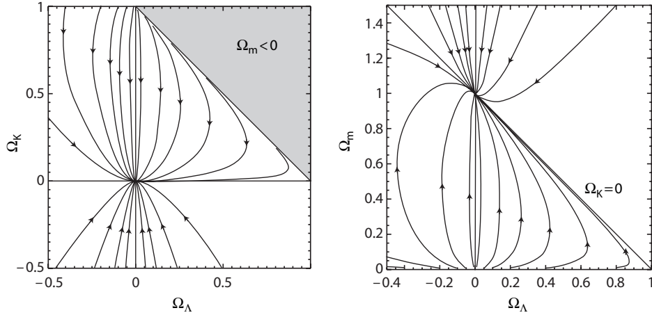
Figure 2.6: Phase space trajectories of the cosmological dynamical system in the (\Omega_K, \Omega_\Lambda) plane (left) and (\Omega_m, \Omega_\Lambda) plane (right) for a phantom / vacuum fluid ( \gamma = 0, w = -1 ).
