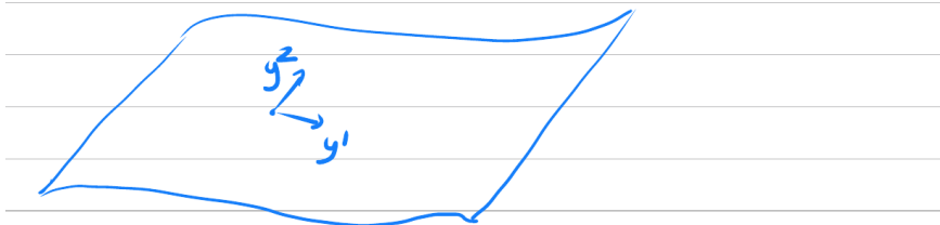
Figure 8.1: Geometric structure of an embedded 2D hypersurface \Sigma in spacetime. The intrinsic coordinates (y^1, y^2) define the tangent basis vectors e_1^a = \frac{\partial x^a}{\partial y^1} and e_2^a = \frac{\partial x^a}{\partial y^2} , while the normal 1-form n_a satisfies n_a e_\mu^a = 0 .
