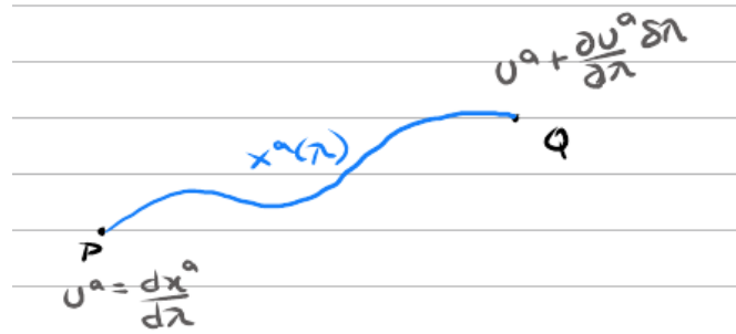
Figure 12.2: Parallel transport of a tangent vector along a curve x^a(\lambda) connecting P to Q .
