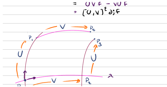
Figure 21.2: Geometric quadrilateral formed by the flows of vector fields u and v . The failure of the loop to close ( P_4 \neq P_3 ) measures the Lie commutator [u, v] .
