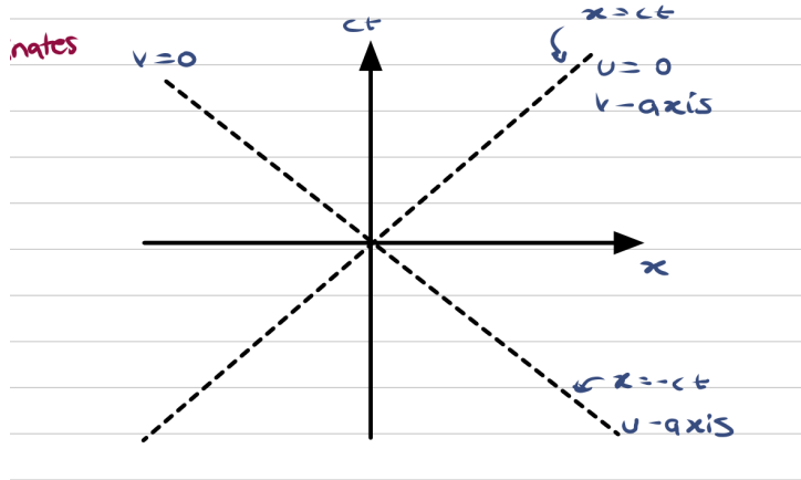
Figure 2.2: Null coordinates (u, v) in Minkowski spacetime. The line u = 0 corresponds to x = ct (the v -axis, outgoing light rays), while v = 0 corresponds to x = -ct (the u -axis, ingoing light rays).
