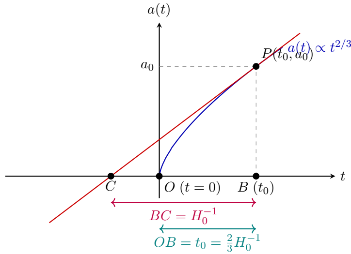
Figure 26.1: Geometric derivation of the cosmic age t_0 for a matter-dominated flat universe. The slope of the tangent line at P(t_0, a_0) is \dot{a}_0 , intercepting the time axis at point C . The distance BC = a_0/\dot{a}_0 = H_0^{-1} represents the Hubble time, yielding t_0 = OB = \frac{2}{3}BC = \frac{2}{3}H_0^{-1} .
