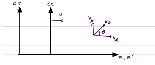
Figure 2.3: Relativistic velocity transformation and aberration. A particle (or light ray) moving with speed v_0 at an angle \theta relative to the boost direction appears at a different angle \theta' in the moving frame.
