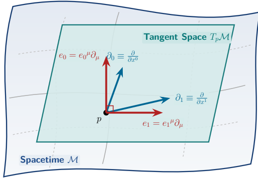
(a) Tangent Space & Vierbein
