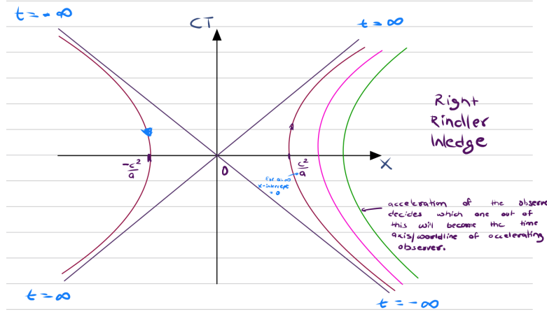
Figure 6.1: The Right Rindler Wedge ( X > |cT| ) in Minkowski spacetime. Hyperbolas of constant x represent the worldlines of stationary accelerated observers with different proper accelerations. The light cone rays X = \pm cT form the asymptotes ( t \rightarrow \pm\infty ).
