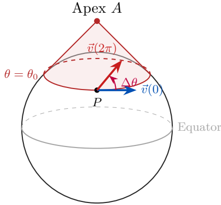
(a) Tangent Cone on S^2
