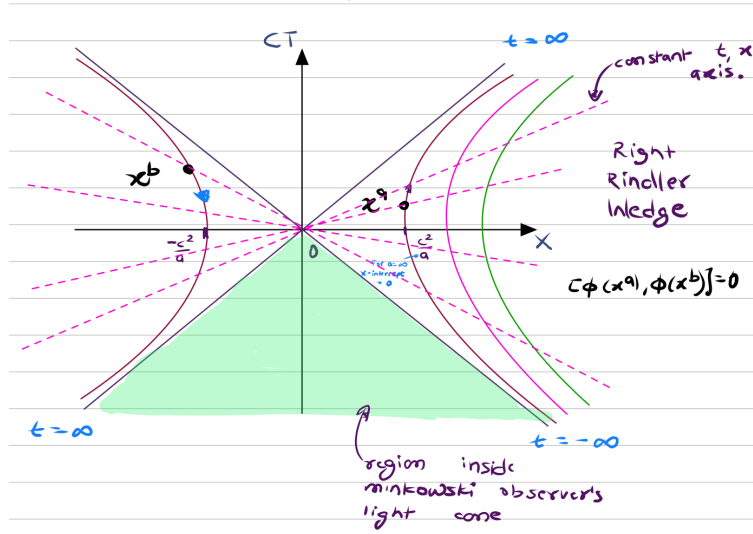
Figure 6.2: Spacetime structure of the Right Rindler Wedge ( X > |cT| ). Dashed magenta lines through the origin represent hypersurfaces of constant accelerated time t = \text{const} . The green shaded region is inside the past light cone. Events x^a and x^b are spacelike separated across the Rindler horizon, ensuring the field commutator vanishes: [\phi(x^a), \phi(x^b)] = 0 .
