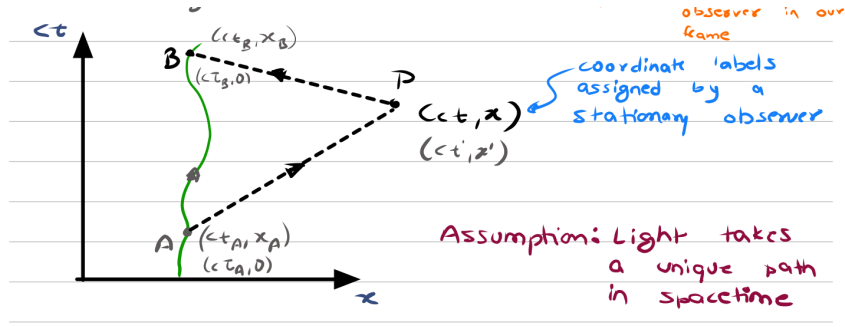
Figure 2.1: Radar coordinate assignment for an arbitrary observer. A light signal emitted at proper time \tau_A bounces off event P and returns to the observer at proper time \tau_B . The observer assigns coordinates (ct', x') based on these emission and reception times.
