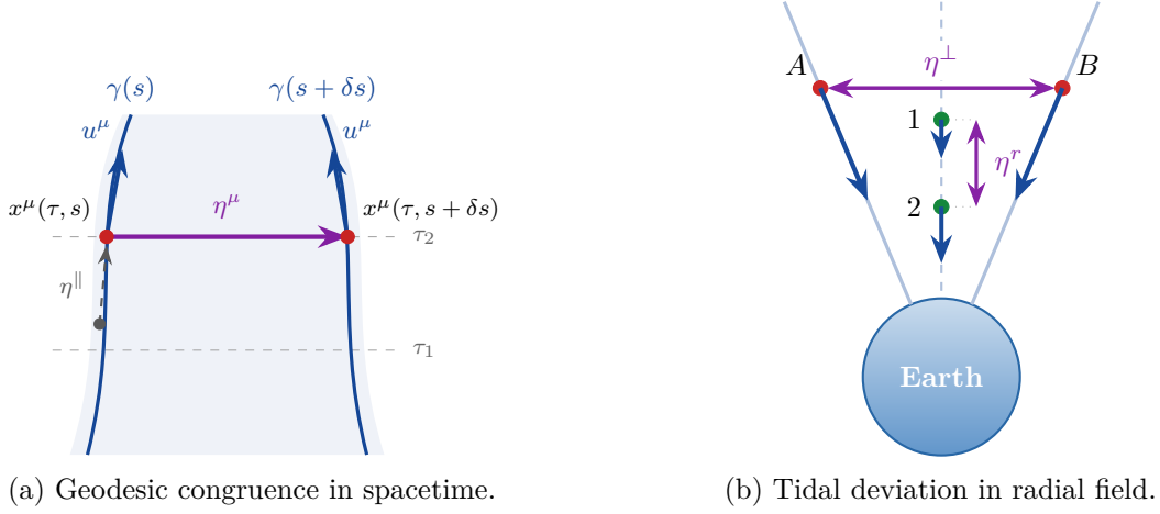
Figure 14.2: Geodesic deviation: (a) congruence geometry, and (b) tidal deviation in Earth's radial field.
