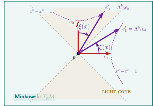
(b) Local Lorentz Gauge Freedom
