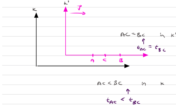
Figure 1.1: Relativity of simultaneity thought experiment. A light source at midpoint C emits signals toward detectors A and B . In frame K' , the events are simultaneous ( t'_{AC} = t'_{BC} ). In frame K , relative motion causes the signals to arrive at different times ( t_{AC} < t_{BC} ).
