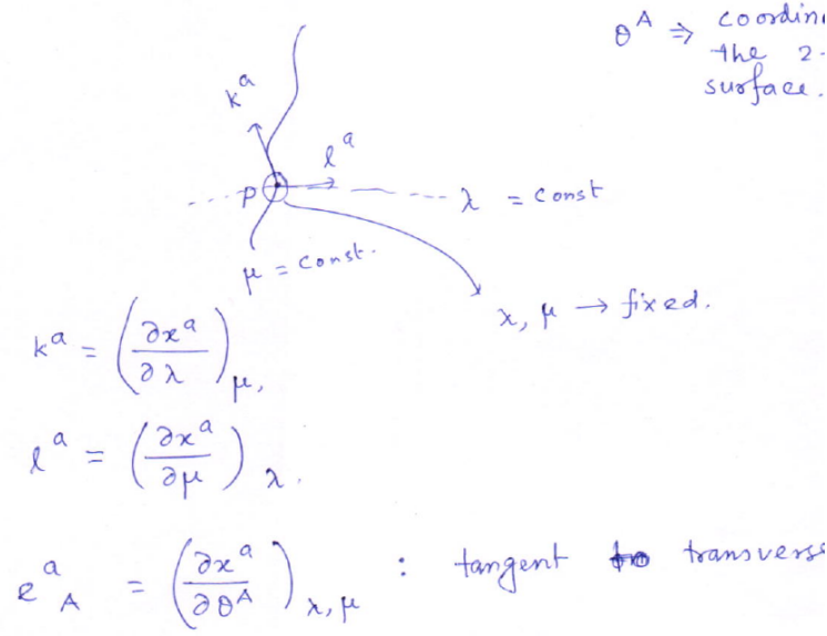
Figure 22.3: Two-dimensional transverse cross-section spanned by coordinates \theta^A , showing the null generators k^a = (\partial x^a / \partial \lambda) and transverse connecting vectors e_A^a = (\partial x^a / \partial \theta^A) .
