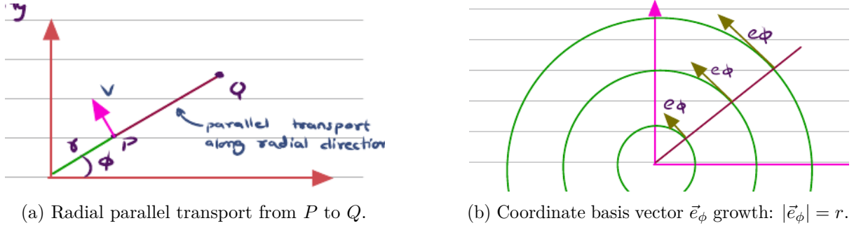
Figure 12.3: Parallel transport in polar coordinates: radial transport and coordinate basis scaling.
