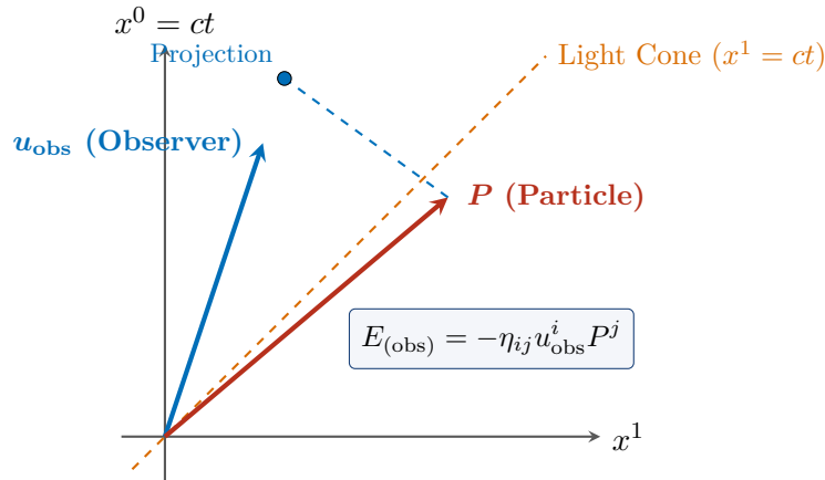
Figure 5.1: Geometric interpretation of energy: the energy of a particle measured by an observer is the invariant projection of the particle's 4-momentum \mathbf{P} along the observer's timelike 4-velocity \mathbf{u}_{\text{obs}} .
