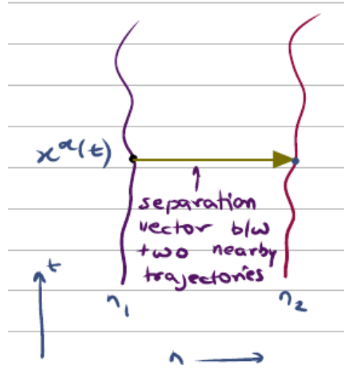
Figure 13.2: Newtonian separation vector \eta^\alpha(t) = \frac{\partial x^\alpha}{\partial n} connecting two neighboring freely falling trajectories.
