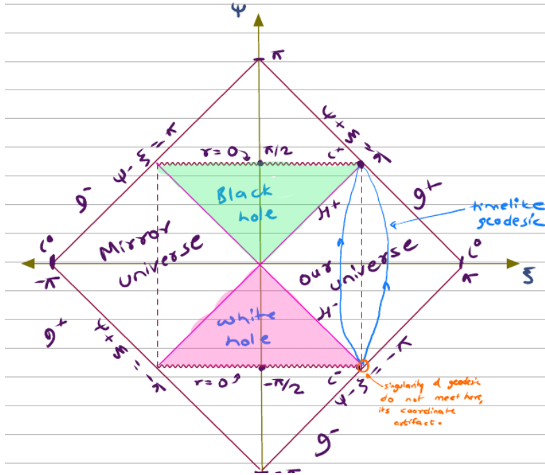
Figure 23.3: Penrose–Carter conformal diagram of the maximally extended Schwarzschild geometry. Light cones are oriented at precisely \pm 45^\circ . Boundaries include: future/past null infinity \mathcal{I}^+, \mathcal{I}^- ; future/past timelike infinity i^+, i^- ; spatial infinity i^0 ; future/past event horizons \mathcal{H}^+, \mathcal{H}^- ; and the physical spacelike singularities r = 0 at \psi = \pm\pi/2 .
