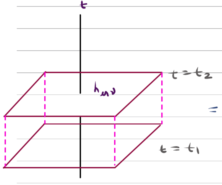
Figure 11.1: Spacetime integration volume \mathcal{M} bounded by two spacelike Cauchy surfaces \Sigma(t_1) and \Sigma(t_2) (with induced 3-metric h_{\mu\nu} and timelike normals n_0 ) and the spatial boundary cylinder \mathcal{B}_\infty at spatial infinity ( r \rightarrow \infty ).
