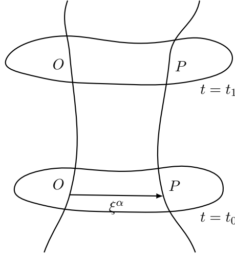
Figure 22.1: Two-dimensional deformable medium and connecting vector \xi^\alpha evolving along worldlines between t = t_0 and t = t_1 .
