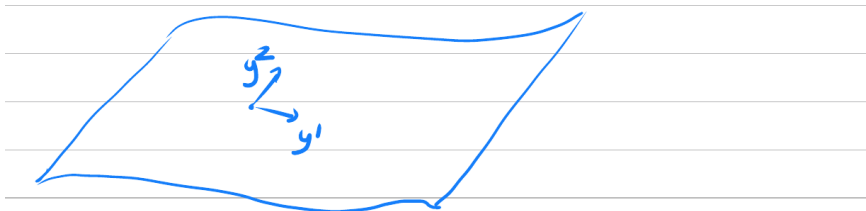
Figure 8.1: Geometric structure of an embedded 2D hypersurface \Sigma in spacetime. The intrinsic coordinates (y^1, y^2) define the tangent basis vectors e_1^a = \frac{\partial x^a}{\partial y^1} and e_2^a = \frac{\partial x^a}{\partial y^2} , while the normal 1-form n_a satisfies n_a e_\mu^a = 0 .
