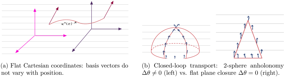
Figure 12.1: Geometric distinction between parallel transport in flat vs. curved manifolds.
