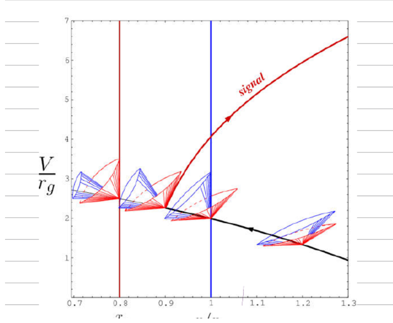
Figure 23.1: Lightcone tilting across the event horizon in ingoing Eddington–Finkelstein coordinates (v/r_g, r/r_g) . For r > r_g = 2GM , outgoing rays escape to infinity ( dr/dv > 0 ). At the horizon r = r_g , outgoing light rays are trapped at dr/dv = 0 , making the horizon a null hypersurface. For r < r_g , both the ingoing and outgoing null boundaries of the lightcone point strictly inward toward decreasing r , forcing all physical trajectories into the central curvature singularity at r = 0 .
