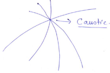
Figure 22.2: Gravitational focusing and the formation of a caustic (conjugate point). Due to the universal non-linear attraction \frac{d\theta}{d\tau} \leq -\frac{1}{3}\theta^2 , neighboring geodesics in an initially converging congruence are focused to a mutual intersection in a finite proper time \tau \leq \frac{3}{|\theta_0|} , at which point the expansion diverges \theta \rightarrow -\infty and the congruence develops an envelope singularity.
