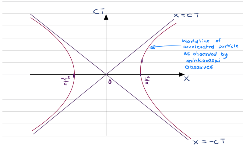
Figure 5.2: Hyperbolic worldline of a uniformly accelerated particle in Minkowski spacetime (cT, X) . The asymptotes X = \pm cT define the causal horizon of the accelerated observer, who remains entirely within the Right Rindler Wedge ( X > |cT| ).
