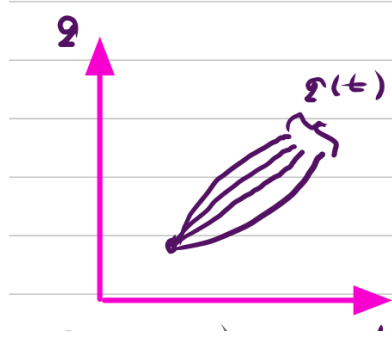
Figure 4.1: On-shell action variation with a variable endpoint q(t) . The bundle of trajectories satisfies the classical Euler–Lagrange equations of motion, so the variation of the action is governed entirely by the boundary terms.
