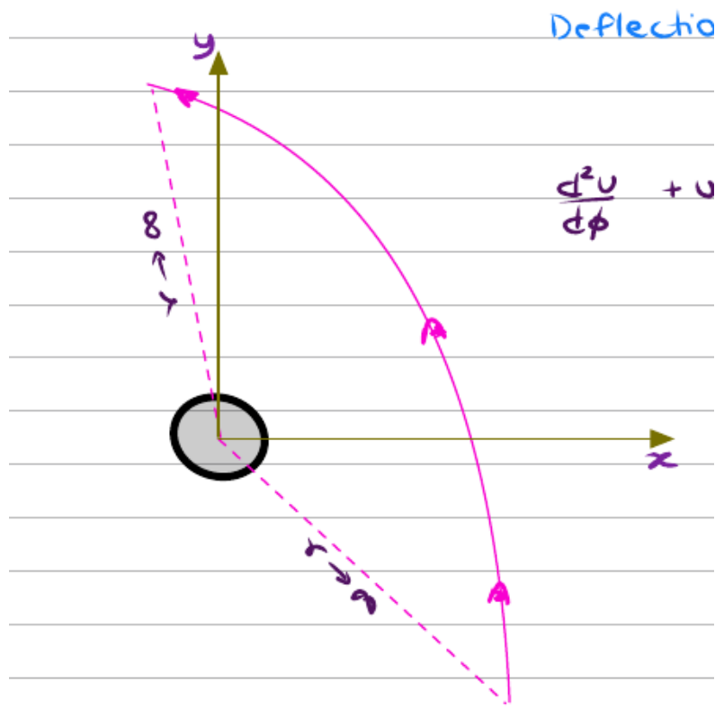
Figure 25.1: Gravitational bending of light rays grazing a mass M with impact parameter b , illustrating the unperturbed asymptote and the total deflection angle \Delta\theta = 4GM/c^2b .
