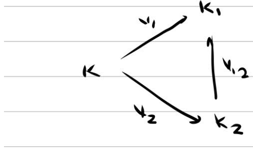
Figure 1.2: Three-frame composition configuration. Frame K observes frames K_1 and K_2 moving with velocities \vec{v}_1 and \vec{v}_2 . The relative velocity between K_1 and K_2 is \vec{v}_{12} .
