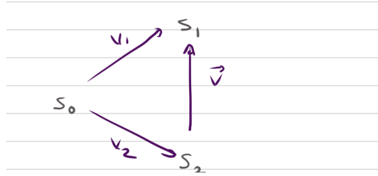
Figure 3.1: Three inertial reference frames S_0, S_1, S_2 . Frame S_0 observes frames S_1 and S_2 moving with velocities \vec{v}_1 and \vec{v}_2 . The vector \vec{v} represents the relative velocity of S_2 measured in the rest frame of S_1 .
