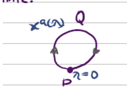
Figure 12.4: Parallel transport around an infinitesimal closed circuit \mathcal{C} .
