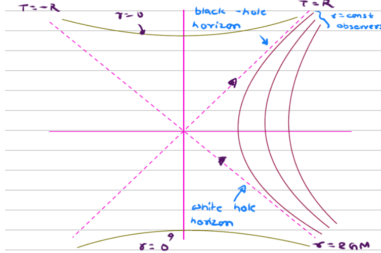
Figure 23.2: The Kruskal–Szekeres diagram representing the maximal analytic extension of Schwarzschild spacetime. Radial null rays travel at strictly \pm 45^\circ . The four distinct spacetime regions are: Region I (our exterior universe, R > |T| ), Region II (future black hole interior, T > |R| ), Region III (parallel mirror universe, R < -|T| ), and Region IV (past white hole interior, T < -|R| ). The physical singularities are hyperbolae at T^2 - R^2 = 1 ( r = 0 ), while future/past horizons are the null lines T = \pm R ( r = 2GM ).
