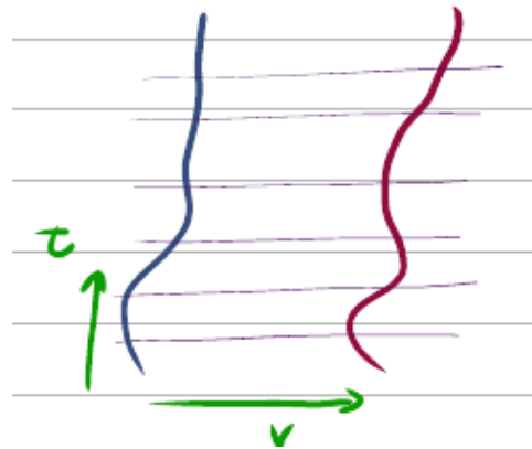
Figure 13.3: A 2-parameter geodesic congruence sheet x^i(\tau, s) with tangent velocity vector u^i = \frac{\partial x^i}{\partial \tau} along the flow and geodesic deviation separation vector v^i = \frac{\partial x^i}{\partial s} across neighboring geodesics.
