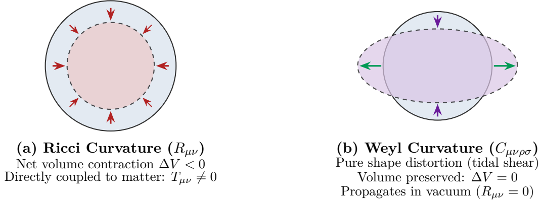
Figure 14.1: Curvature decomposition on a cloud of freely falling particles: (a) Ricci volume compression vs. (b) Weyl tidal shape deformation.
