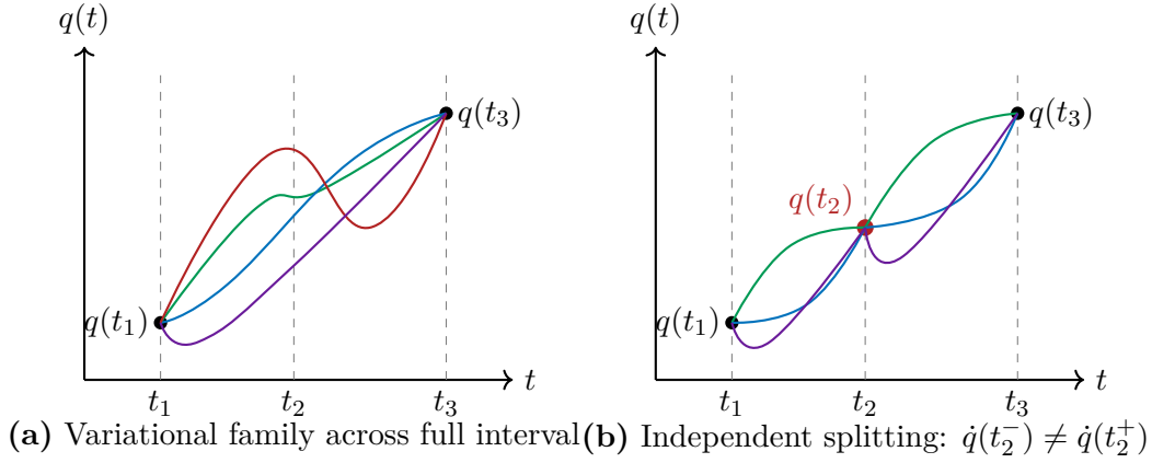
Figure 15.1: Action decomposition across intermediate boundary t_2 . If derivative variations \delta\dot{q} are arbitrarily constrained at intermediate surfaces, non-differentiable trajectory kinks ( \dot{q}(t_2^-) \neq \dot{q}(t_2^+) ) are artificially introduced.
