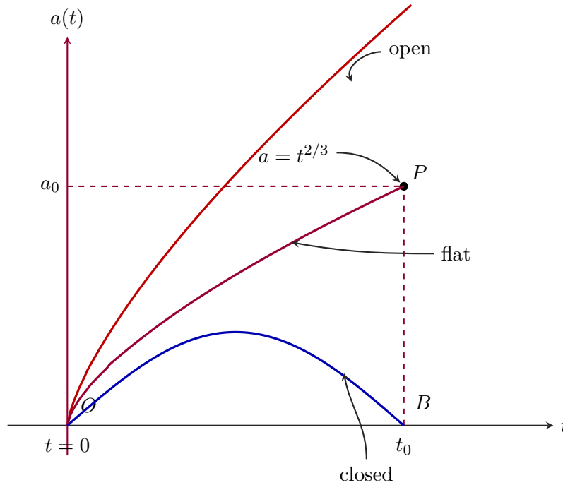
Figure 26.2: Comparative dynamical evolution of the cosmic scale factor a(t) for matter-dominated open ( k = -1 ), flat ( k = 0, a \propto t^{2/3} ), and closed ( k = +1 ) universes, exactly matching the structure of the lecture notes. The flat curve passes through (t_0, a_0) at point P . The open curve expands fastest and remains above the flat curve, while the closed model reaches a maximum and recollapses to zero size at point B(t_0) .
