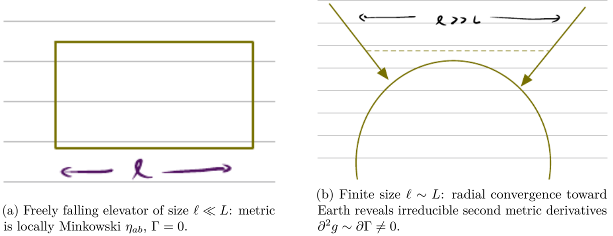
Figure 13.1: The physical limit of the Equivalence Principle and the onset of tidal gravitational forces.
