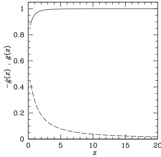
Figure 6.15: The gravitational potential growth function g(z) (solid line) and its time derivative \dot{g}(z) (dashed line) as functions of redshift in a flat \Lambda CDM universe with \Omega_{\Lambda} = 0.7 and \Omega_m = 0.3 . Notice that g(z) deviates significantly from unity only at late times ( z \lesssim 2 ) when dark energy dominates.
