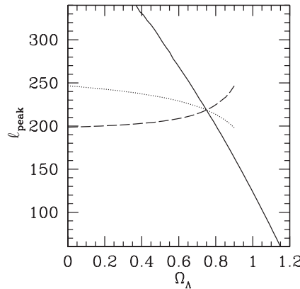
Figure 6.1: The position of the first acoustic peak \ell_1 as a function of \Omega_\Lambda . Solid line: varying \Omega_K while leaving all other parameters fixed. Dashed line: varying \Omega_\Lambda at fixed h = 0.72 . Dotted line: varying \Omega_\Lambda at fixed \Omega_m h^2 . The fixed baseline parameters are \Omega_K = 0, h = 0.72, \Omega_b h^2 = 0.022, \Omega_m = 0.25, n_s = 0.96, \tau_{\text{ri}} = 0.085 , so that all curves intersect at \Omega_\Lambda = 0.75 . Notice the pronounced sensitivity of \ell_1 to spatial curvature.
