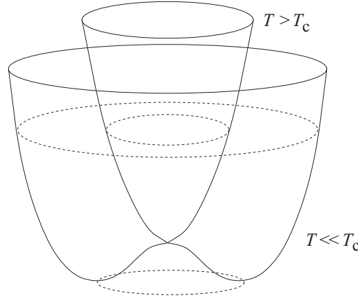
Figure 6.18: The finite-temperature effective potential V(\phi, T) of a complex Higgs field for T > T_c (single symmetric vacuum) and T \ll T_c (spontaneously broken U(1) symmetry with vacuum manifold \mathcal{S}^1 ).
