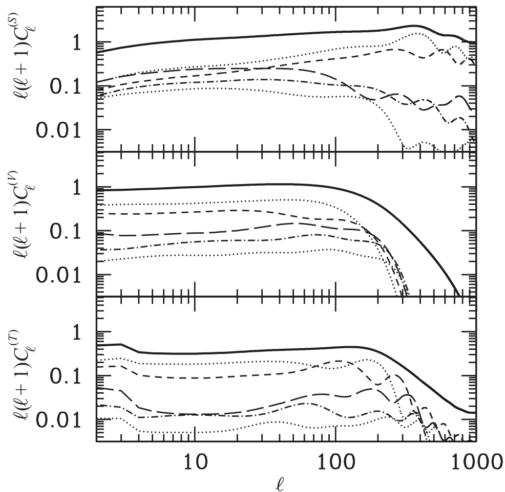
Figure 6.21: The scalar ( S ), vector ( V ), and tensor ( T ) contributions to the CMB temperature power spectrum \ell(\ell+1)C_\ell for a 4-component global texture model. Dashed curves indicate contributions from individual single eigenfunctions, while the bold solid curve shows their total sum over 100 modes. While individual eigenmodes display oscillations, they wash out into a broad hump in the sum (data courtesy of Bevis et al., 2004).
