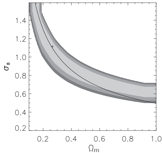
Figure 6.17: Cosmological constraints in the (\Omega_m, \sigma_8) plane from cosmic shear measurements (Maoli et al., 2001). The light, medium, and dark shaded regions enclose the 1\sigma , 2\sigma , and 3\sigma confidence contours. The cross marks the best-fit model, and the solid curve displays the constraint inferred from local galaxy cluster abundances.
