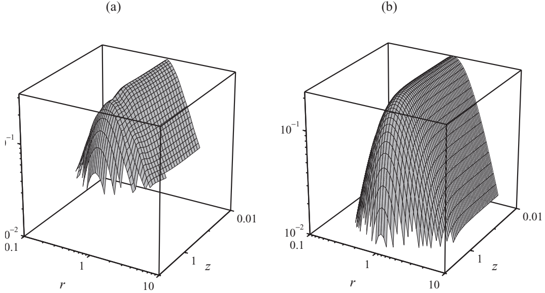
Figure 6.20: The source unequal-time correlation function F(r, z) for vector perturbations as a function of z = k\sqrt{\eta\eta'} and r = t/t' : (a) measured from numerical field simulations of a 4-component global texture, and (b) semi-analytical large- N limit (adapted from Durrer et al., 2002).
