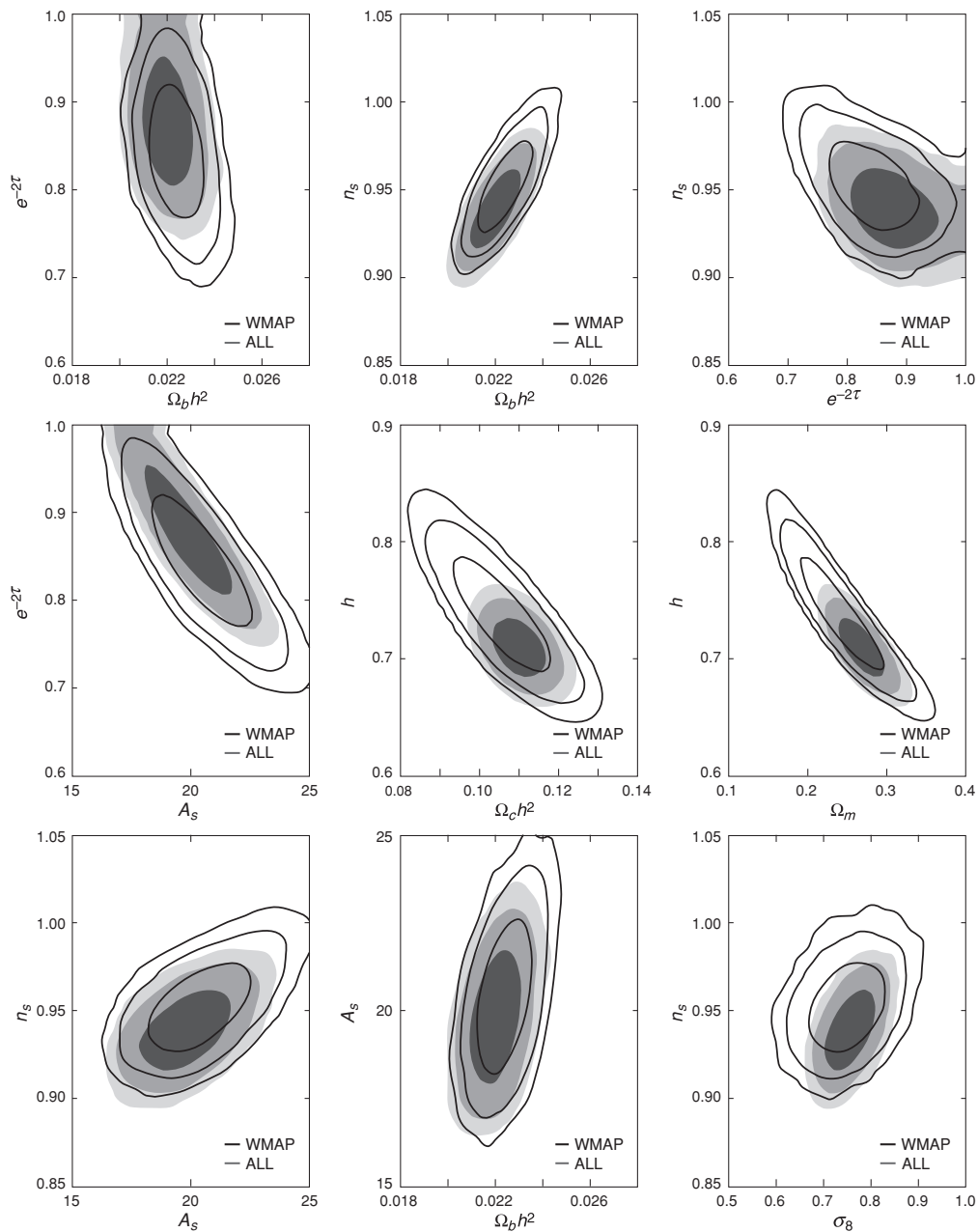
Figure 6.9: Marginalized 2D cosmological parameter posterior distributions from WMAP 3-year data alone (black contours) and combined with small-scale CMB, supernovae, and galaxy surveys (colored contours) for a flat 5-parameter \Lambda CDM model ( \Omega_b h^2, \Omega_{\text{cdm}} h^2, n_s, A_s, \tau ). Figure from Spergel et al. (2007).
