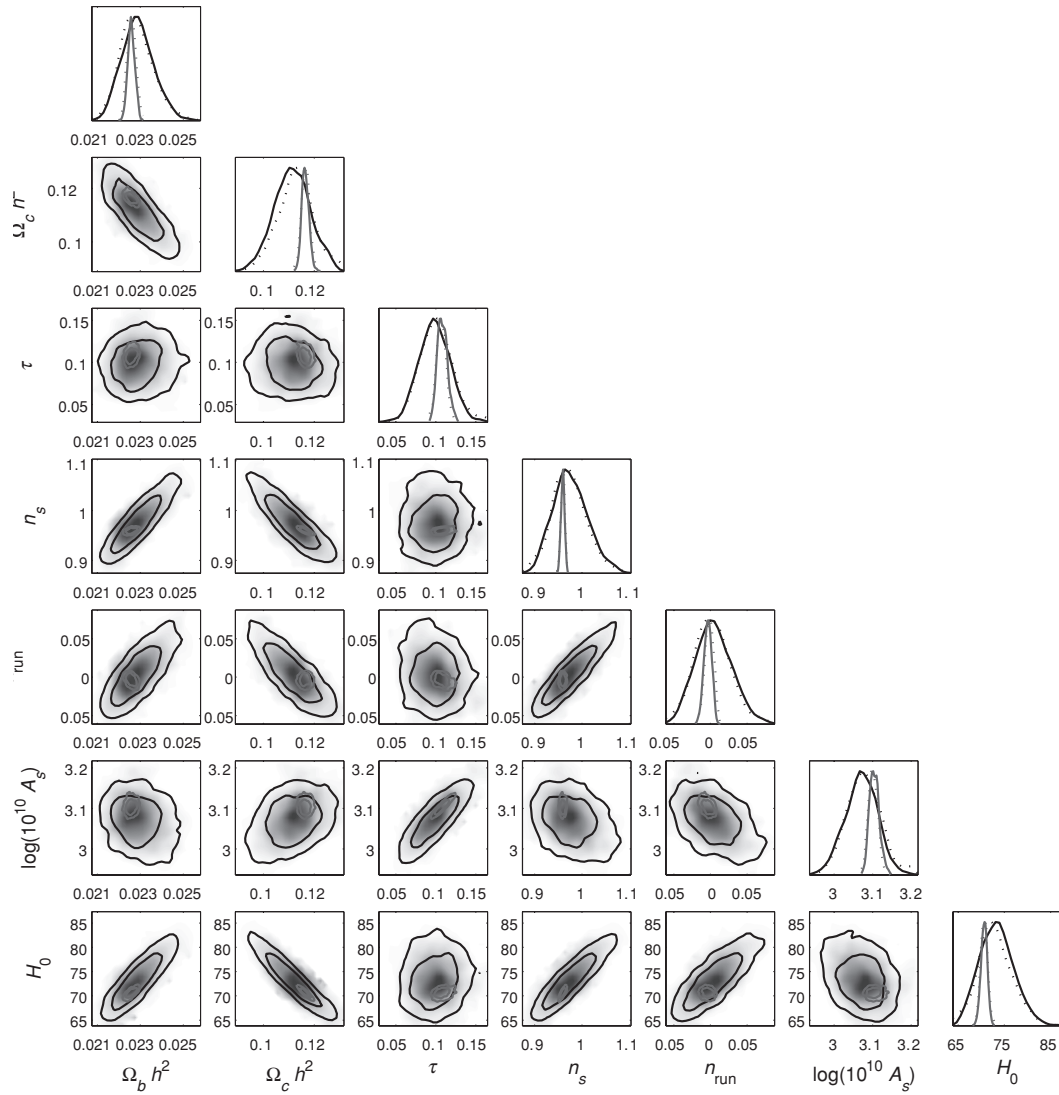
Figure 6.10: Marginalized 1D and 2D parameter probability distributions forecasted for the Planck satellite experiment for a 7-parameter flat model ( \Omega_b h^2, \Omega_{\text{cdm}} h^2, \tau, n_s, n_{\text{run}}, \ln(10^{10} A_s), H_0 ). Figure from ESA (2005).
