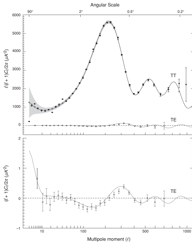
Figure 6.6: The CMB temperature anisotropy power spectrum (TT) and the temperature–polarization cross-correlation spectrum (TE) obtained from the WMAP 3-year data (from Hinshaw et al., 2007).
