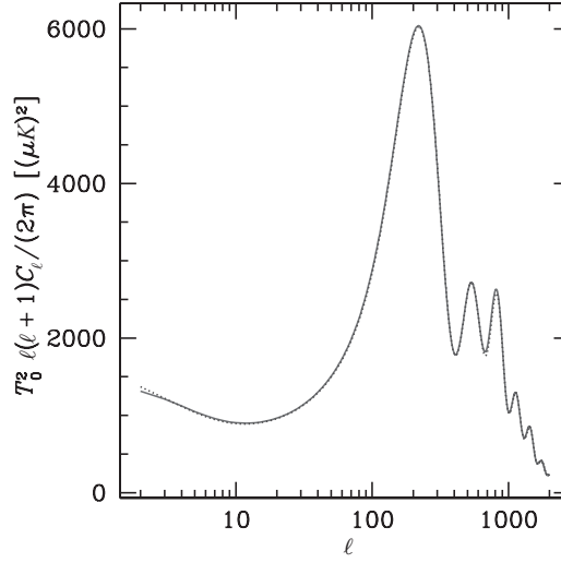
Figure 6.13: Comparison between a purely scalar model with red tilt n_s = 0.96 (solid line) and a model with a significant tensor contribution of r = 0.3 and scale-invariant tilt n_s = 1.0 (dotted line). Both models lie within 1\sigma – 2\sigma of concordance parameters and produce nearly identical temperature power spectra.
