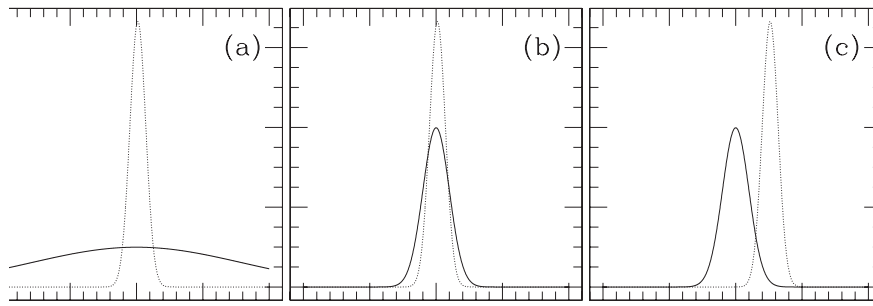
Figure 6.11: Three 1-parameter models with their prior (solid lines) and posterior (dotted curves). All three models have comparable maximum likelihoods. In (a), the prior volume is much wider than the posterior, leading to a small Occam factor. In (b) and (c), the widths are comparable, but model (c) lacks overlap between prior and data. Model (b) has the largest Bayesian evidence.
