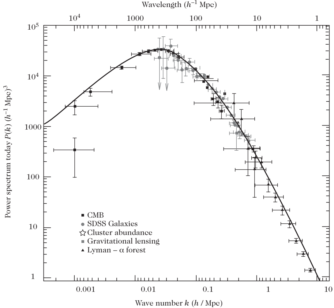
Figure 4.18: The matter power spectrum compared with various observational constraints, ranging from linear scales (cosmic microwave background) to non-linear scales (galaxy surveys, here SDSS), cluster abundances, gravitational lensing, and Lyman- \alpha forests. From Ref. [47].
