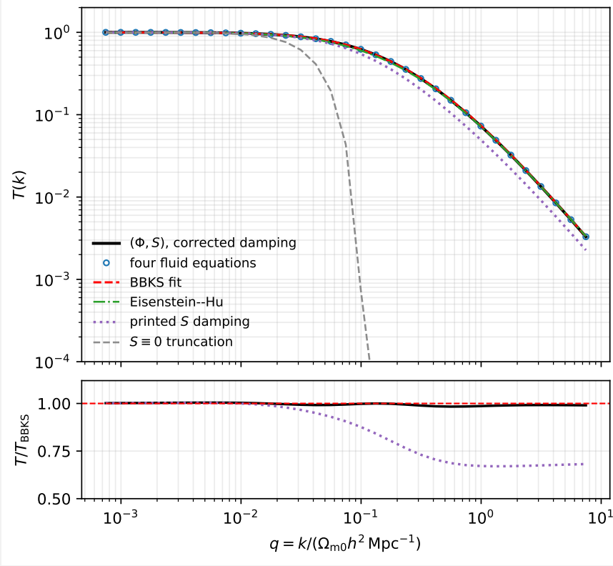
Figure 4.16: Transfer function from the system (11) (solid) and from the fluid equations (6) (circles), against the fitting formula (4.4.42), the Eisenstein–Hu zero-baryon form, the same system integrated with the damping coefficient (3y + 2)/[2y(1 + y)] (dotted), and the truncation S \equiv 0 (grey dashed). Lower panel: ratio to (4.4.42).
