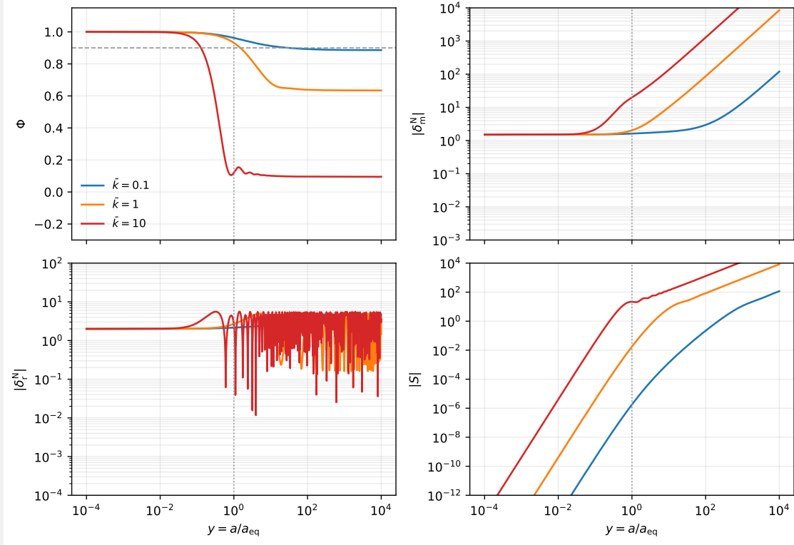
Figure 4.15: Variables of the system (11) and the fluid contrasts reconstructed from (16), for \bar{k} = 0.1, 1, 10 . The dotted vertical line marks equality; the dashed line in the first panel is the super-Hubble value 9/10 .
