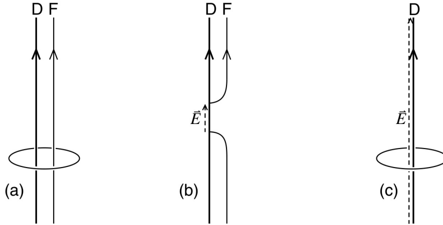
Figure 13.6.1: (a) Parallel D-string and F-string. The loop signifies a 7-sphere surrounding the strings. (b) The F-string breaks, its ends attaching to the D-string. (c) Final state: D-string with flux.
