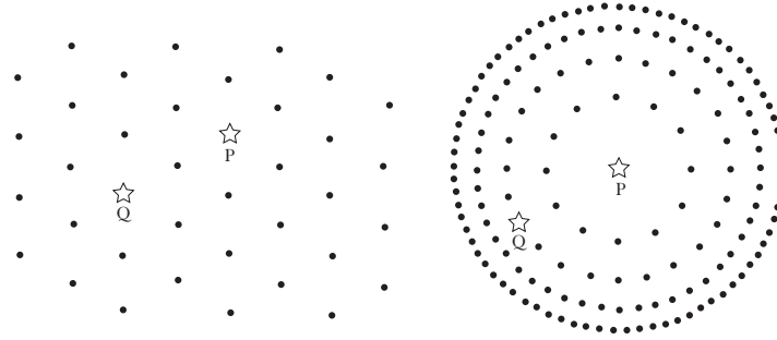
Figure 2.1: Point distributions illustrating uniformity: (Left) Statistically isotropic around every point, implying spatial homogeneity. (Right) Isotropic around a single privileged center P , where points P and Q are physically distinct. The Copernican principle excludes centered models.
