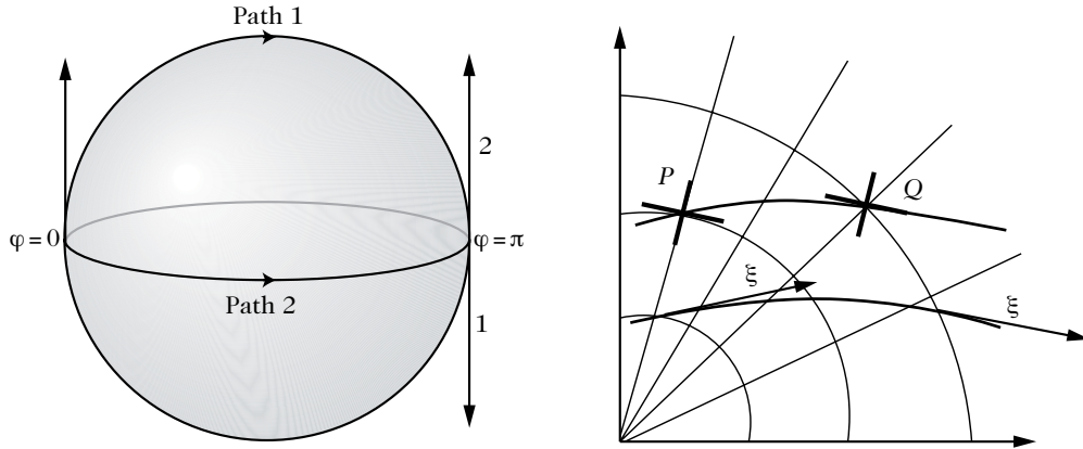
Figure 1.5: (Left): On a 2-dimensional sphere, a vector can be transported parallel to itself along a path 1 corresponding to a great circle until its antipodal point. We can reach the same point following the path 2 along the equator. The two vectors that we get do not coincide. (Right): The Lie derivative evaluates the change determined by an observer that goes from a point P to a point Q along the flow curves of the vector field \xi^\mu transporting its local frame with it.
