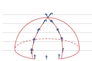
(b) Closed-loop transport: 2-sphere anholonomy \Delta\theta \neq 0 (left) vs. flat plane closure \Delta\theta = 0 (right).
