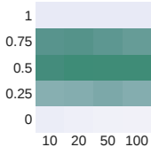
Java
