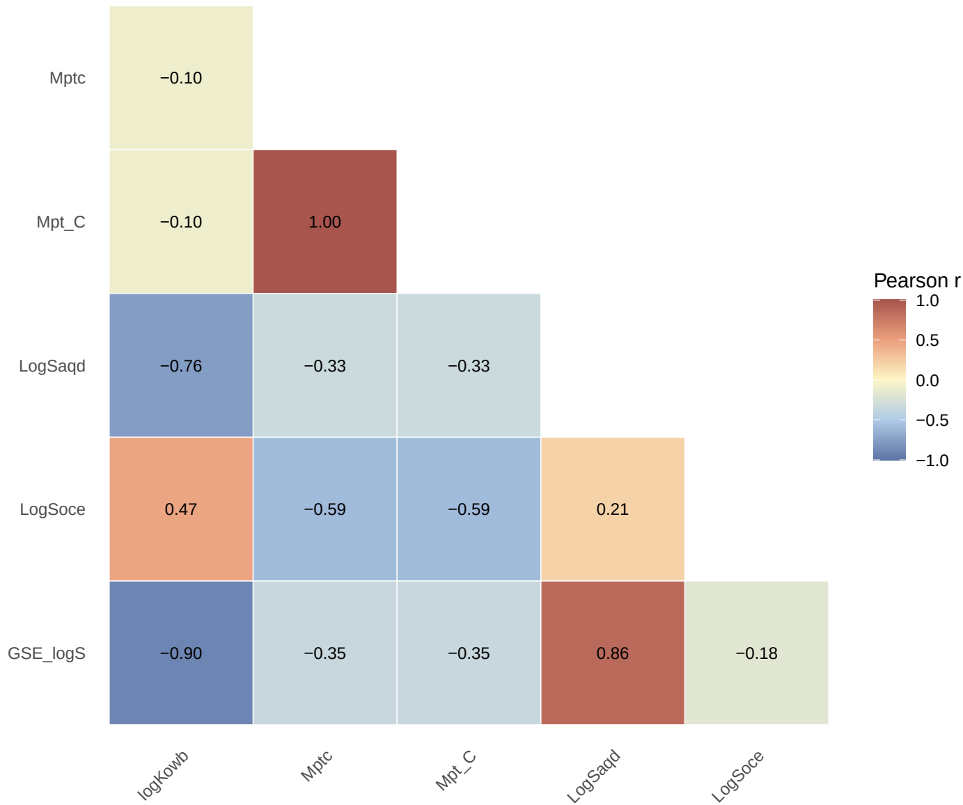
Solubility-related descriptor correlation structure
