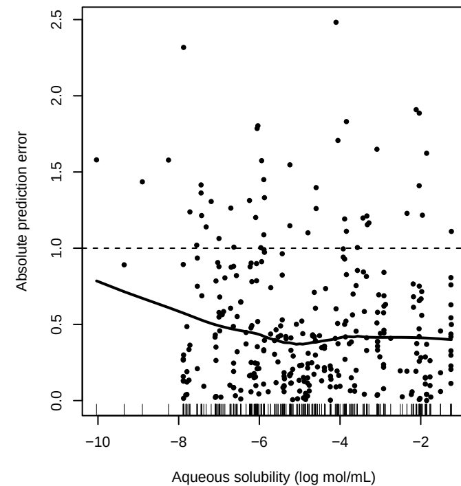
Aqueous solubility
