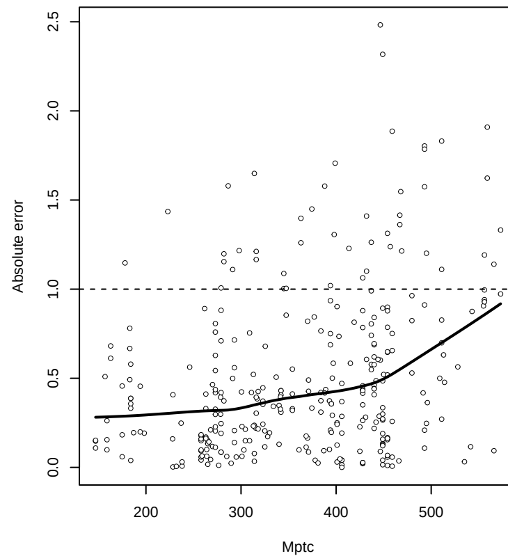
Absolute prediction error by descriptor
