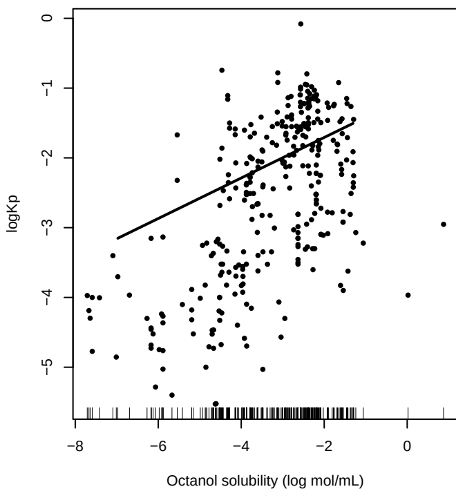
Octanol solubility
