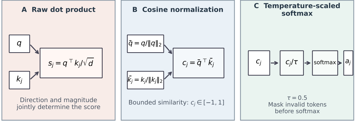
Figure 3: Mechanism of graph-conditioned token attention. Raw dot products combine vector direction and magnitude, cosine normalization bounds the similarity, and temperature-scaled softmax converts normalized scores into masked attention weights. The diagram contains no measured attention values.
