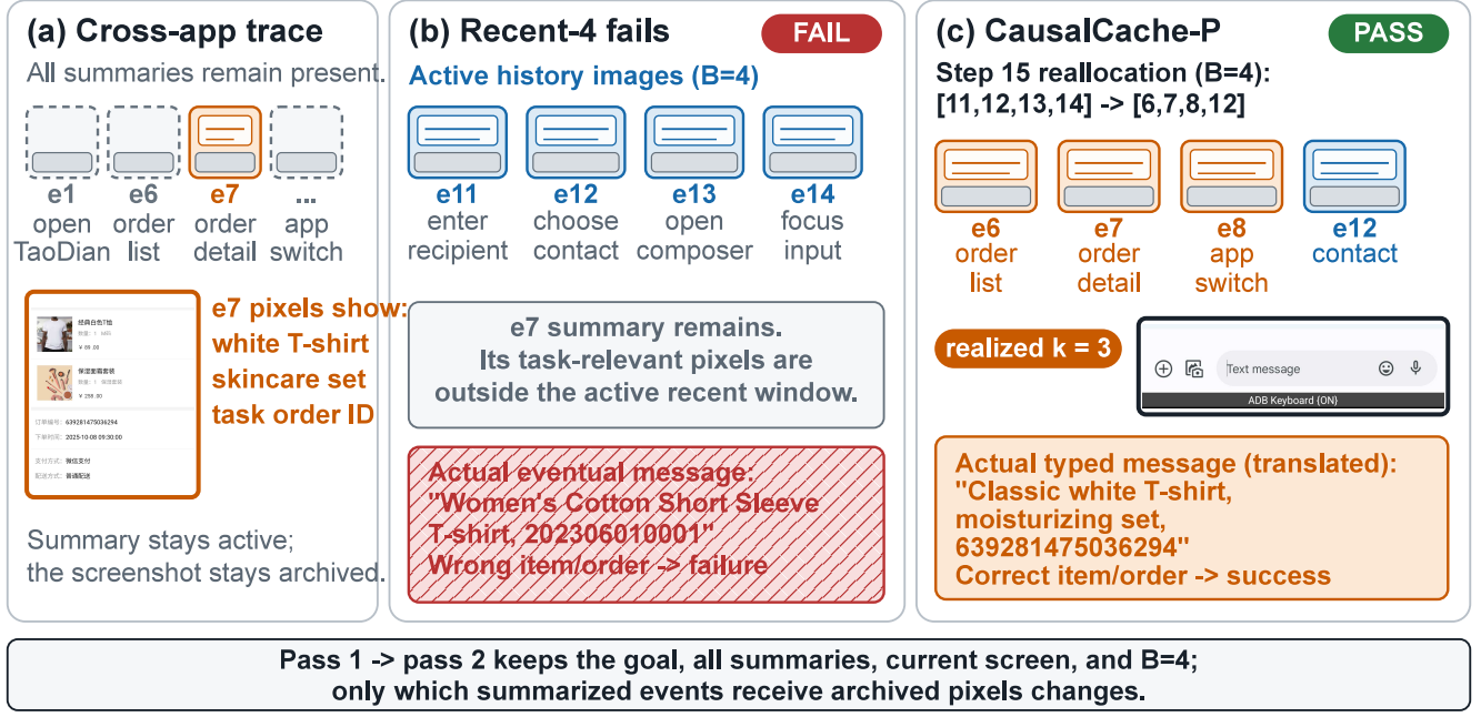
Figure 2: A qualitative cross-app CartInfoNotificationTask case. Both policies retain the complete summary trace and four active history-image slots. At the critical message-composition step, CAUSALCACHE-P reallocates [11, 12, 13, 14] → [6, 7, 8, 12] (realized k=3 ), reattaching the archived order screenshot at event 7. Recent-4 has no product or order pixels and types the wrong values; CAUSALCACHE restores the visual evidence and succeeds. This case illustrates the mechanism; aggregate evidence is reported in text.
