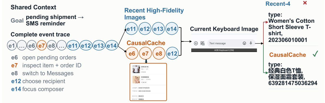
Figure 2: A real cross-app CartInfoNotificationTask episode. The agent must inspect items awaiting shipment in TaoDian, then send an SMS containing only the product names and order number. Both rollouts retain the complete summary trace and use four active history-image slots. Recent-4 exposes [e11, e12, e13, e14] . CAUSALCACHE-P instead exposes [e6, e7, e8, e12] , restoring the enlarged e7 order screenshot before the shared message-composition stage. Recent-4 types the wrong item and order number and fails; CAUSALCACHE types the visually recovered values and succeeds. This single episode illustrates the mechanism rather than an aggregate effect.
