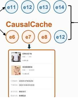
Figure 2: A real cross-app CartInfoNotificationTask episode. The agent must inspect items awaiting shipment in TaoDian, then send an SMS containing only the product names and order number. Both rollouts retain the complete summary trace and use four active history-image slots. Recent-4 exposes [e11, e12, e13, e14] . CAUSALCACHE-P instead exposes [e6, e7, e8, e12] , restoring the enlarged e7 order screenshot before the shared message-composition stage. Recent-4 types the wrong item and order number and fails; CAUSALCACHE types the visually recovered values and succeeds. This single episode illustrates the mechanism rather than an aggregate effect.
